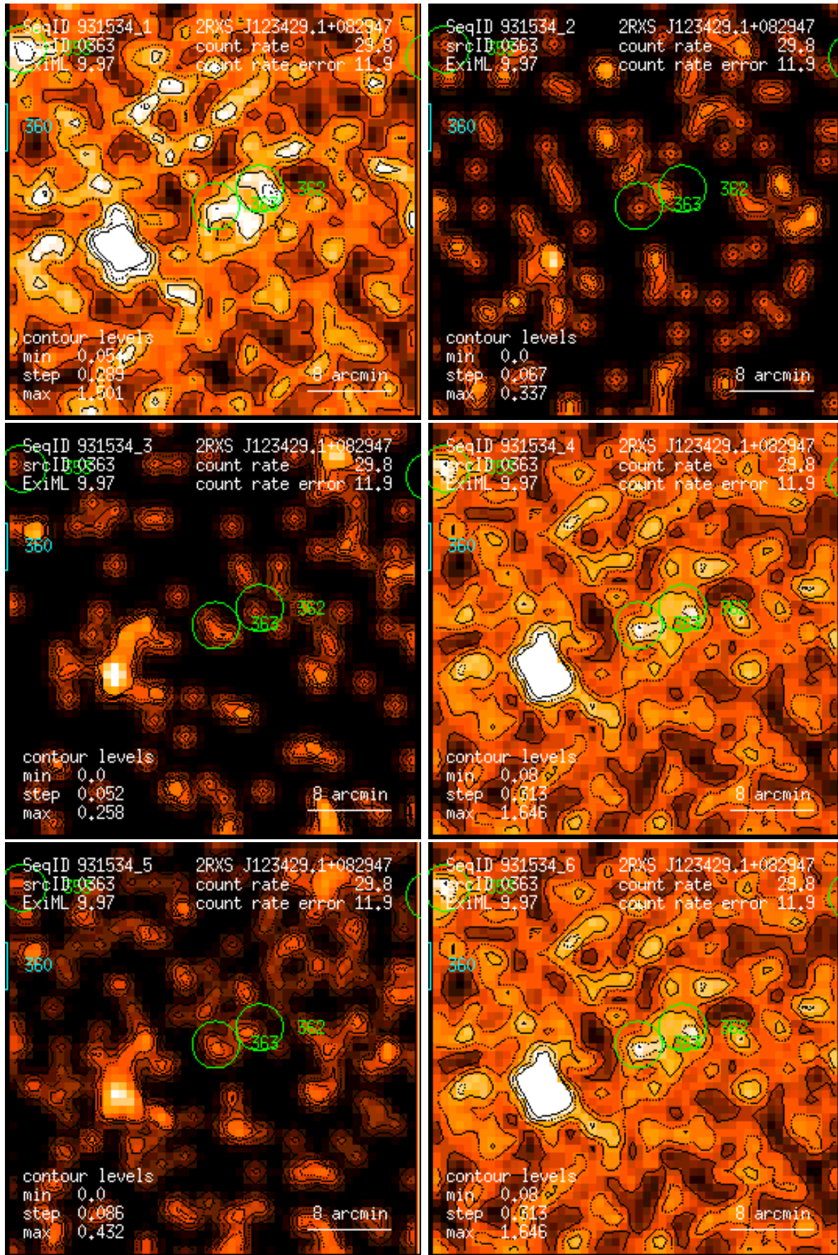
Figure 363: RASS 931534: detection 0363: band rate images, Gaussian filter: (1) PSPC channels 11 – 41, (2) 52 – 90, (3) 91 – 201, (4) 11 – 235, (5) 52 – 201, (6) 11 – 201. Broad band rates in counts/ks. Band rate contour levels in counts/ks/arcmin 2 .
