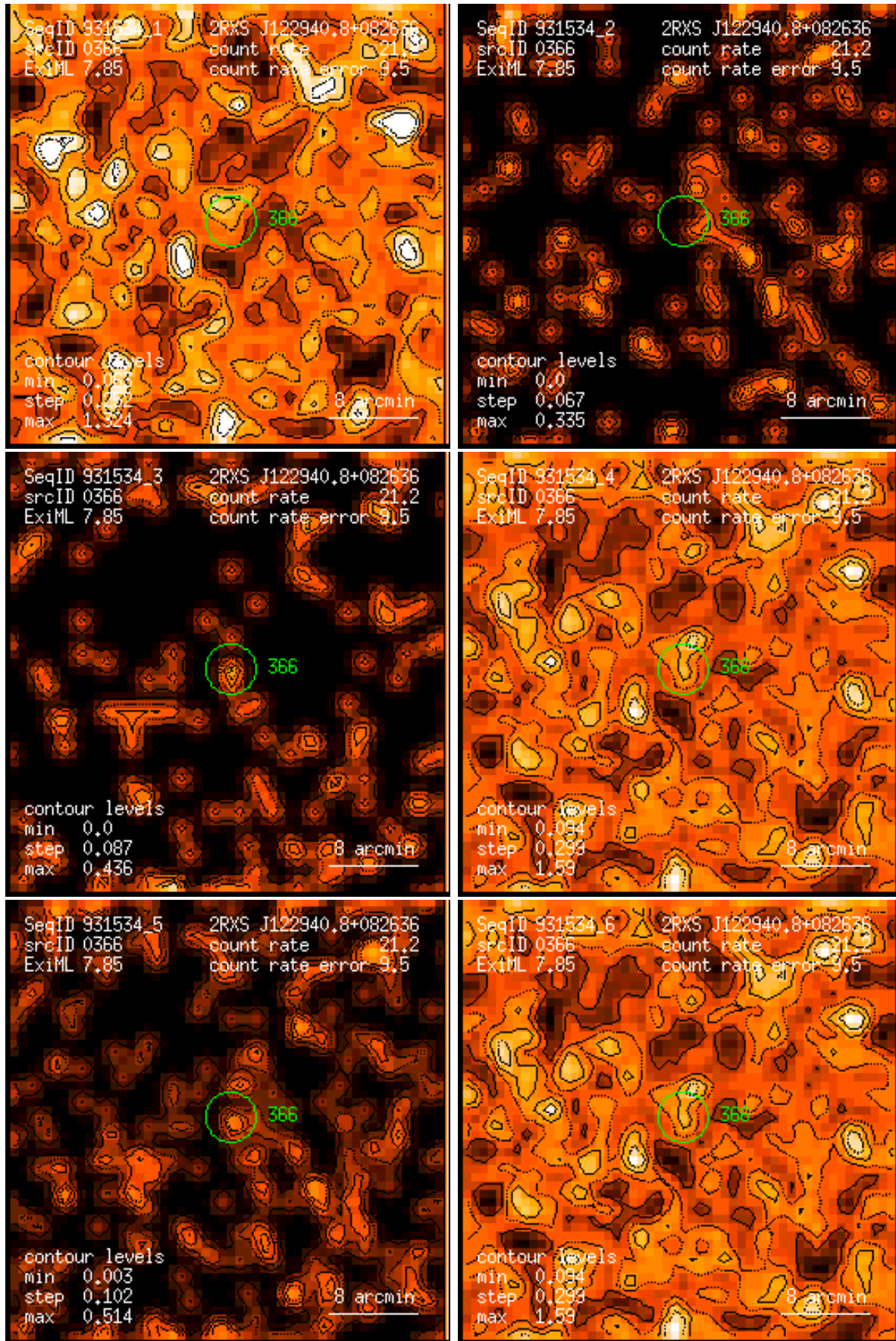
Figure 366: RASS 931534: detection 0366: band rate images, Gaussian filter: (1) PSPC channels 11 – 41, (2) 52 – 90, (3) 91 – 201, (4) 11 – 235, (5) 52 – 201, (6) 11 – 201. Broad band rates in counts/ks. Band rate contour levels in counts/ks/arcmin 2 .
