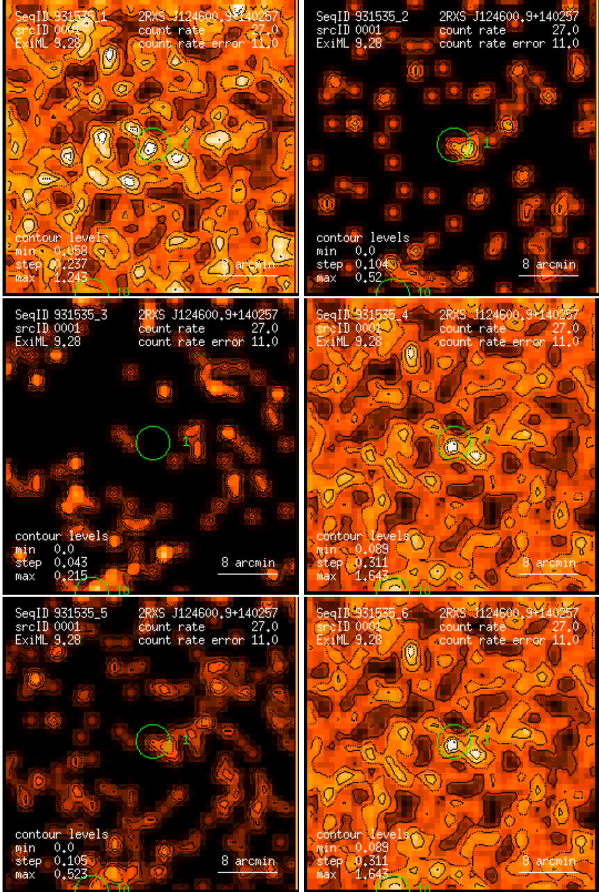
Figure 1: RASS 931535: detection 0001: band rate images, Gaussian filter: (1) PSPC channels 11 – 41, (2) 52 – 90, (3) 91 – 201, (4) 11 – 235, (5) 52 – 201, (6) 11 – 201. Broad band rates in counts/ks. Band rate contour levels in counts/ks/arcmin 2 .
