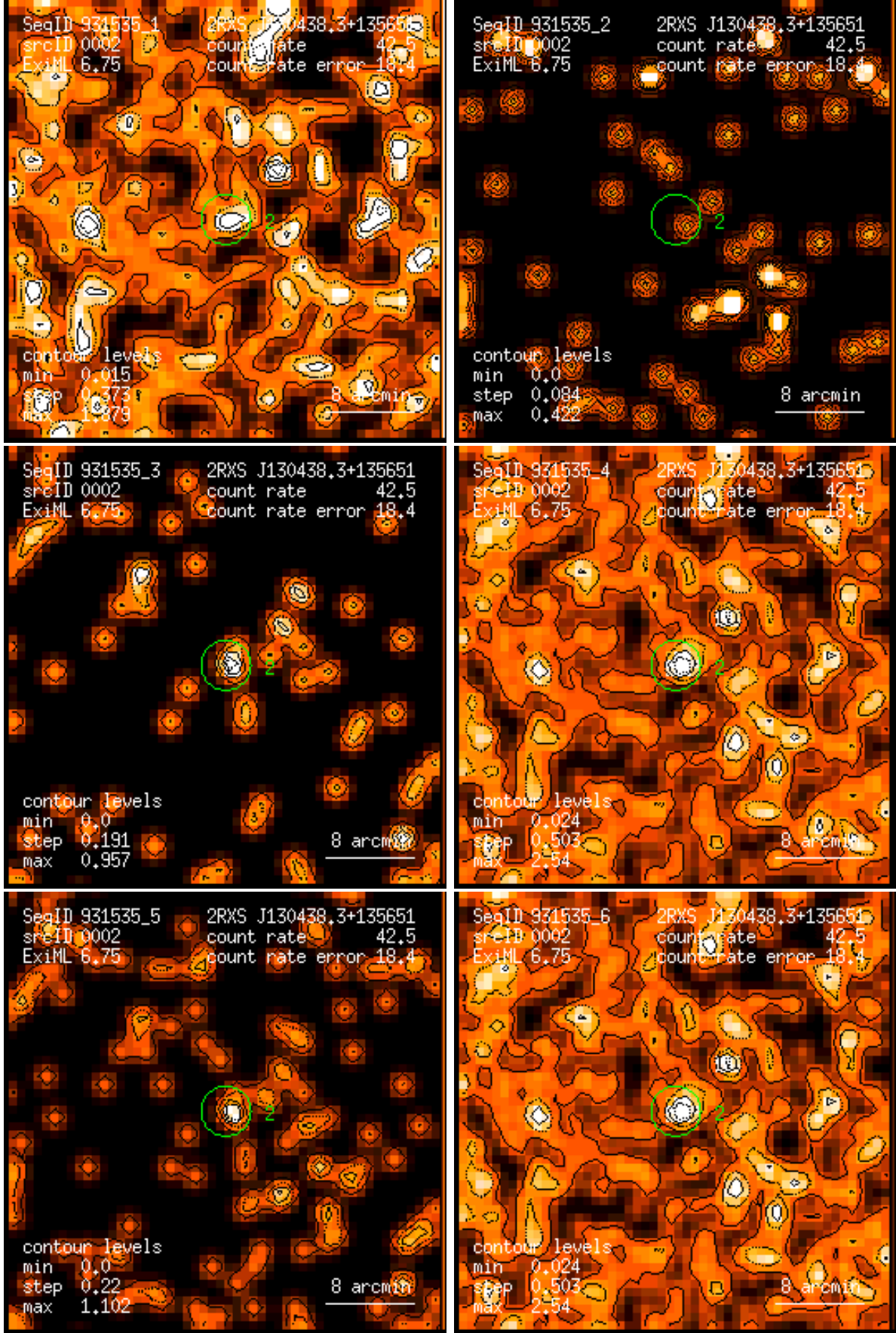
Figure 2: RASS 931535: detection 0002: band rate images, Gaussian filter: (1) PSPC channels 11 – 41, (2) 52 – 90, (3) 91 – 201, (4) 11 – 235, (5) 52 – 201, (6) 11 – 201. Broad band rates in counts/ks. Band rate contour levels in counts/ks/arcmin 2 .
