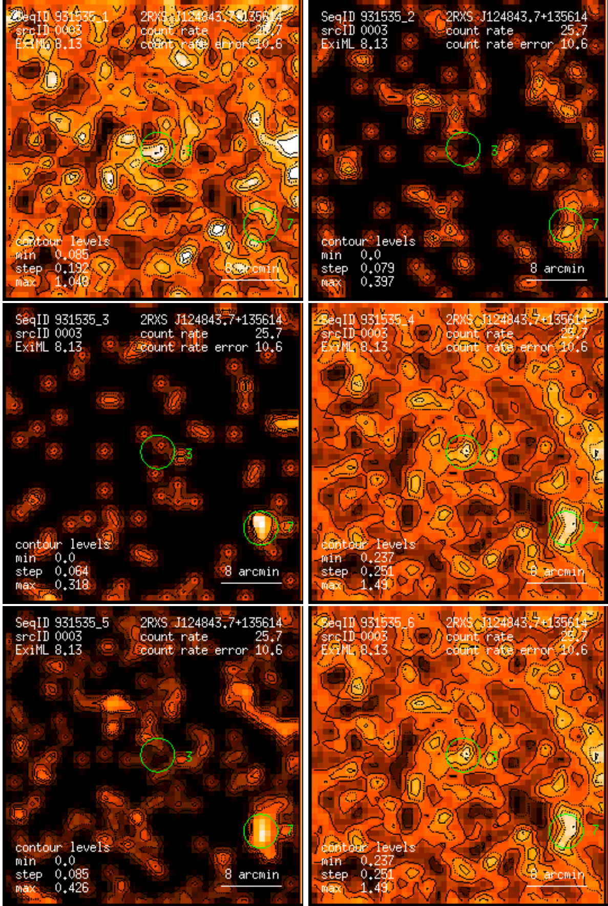
Figure 3: RASS 931535: detection 0003: band rate images, Gaussian filter: (1) PSPC channels 11 – 41, (2) 52 – 90, (3) 91 – 201, (4) 11 – 235, (5) 52 – 201, (6) 11 – 201. Broad band rates in counts/ks. Band rate contour levels in counts/ks/arcmin 2 .
