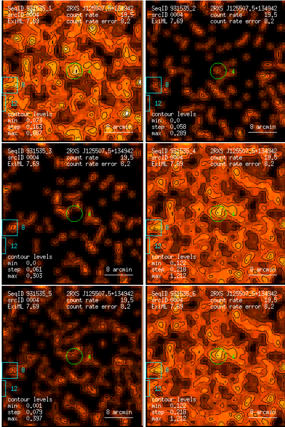
Figure 4: RASS 931535: detection 0004: band rate images, Gaussian filter: (1) PSPC channels 11 – 41, (2) 52 – 90, (3) 91 – 201, (4) 11 – 235, (5) 52 – 201, (6) 11 – 201. Broad band rates in counts/ks. Band rate contour levels in counts/ks/arcmin 2 .
