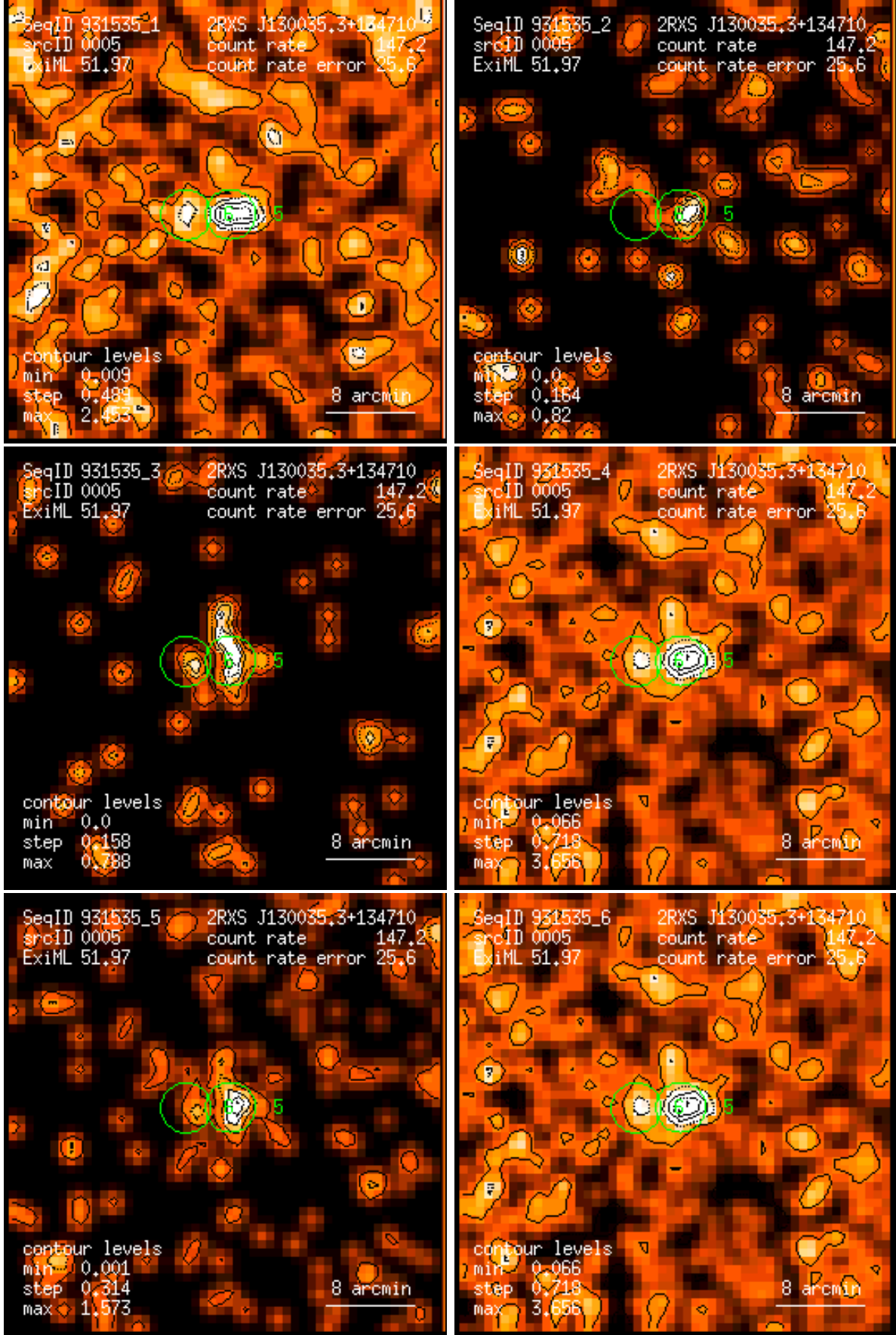
Figure 5: RASS 931535: detection 0005: band rate images, Gaussian filter: (1) PSPC channels 11 – 41, (2) 52 – 90, (3) 91 – 201, (4) 11 – 235, (5) 52 – 201, (6) 11 – 201. Broad band rates in counts/ks. Band rate contour levels in counts/ks/arcmin 2 .
