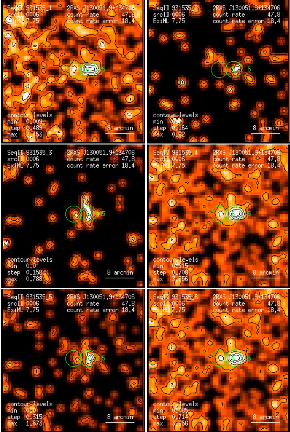
Figure 6: RASS 931535: detection 0006: band rate images, Gaussian filter: (1) PSPC channels 11 – 41, (2) 52 – 90, (3) 91 – 201, (4) 11 – 235, (5) 52 – 201, (6) 11 – 201. Broad band rates in counts/ks. Band rate contour levels in counts/ks/arcmin 2 .
