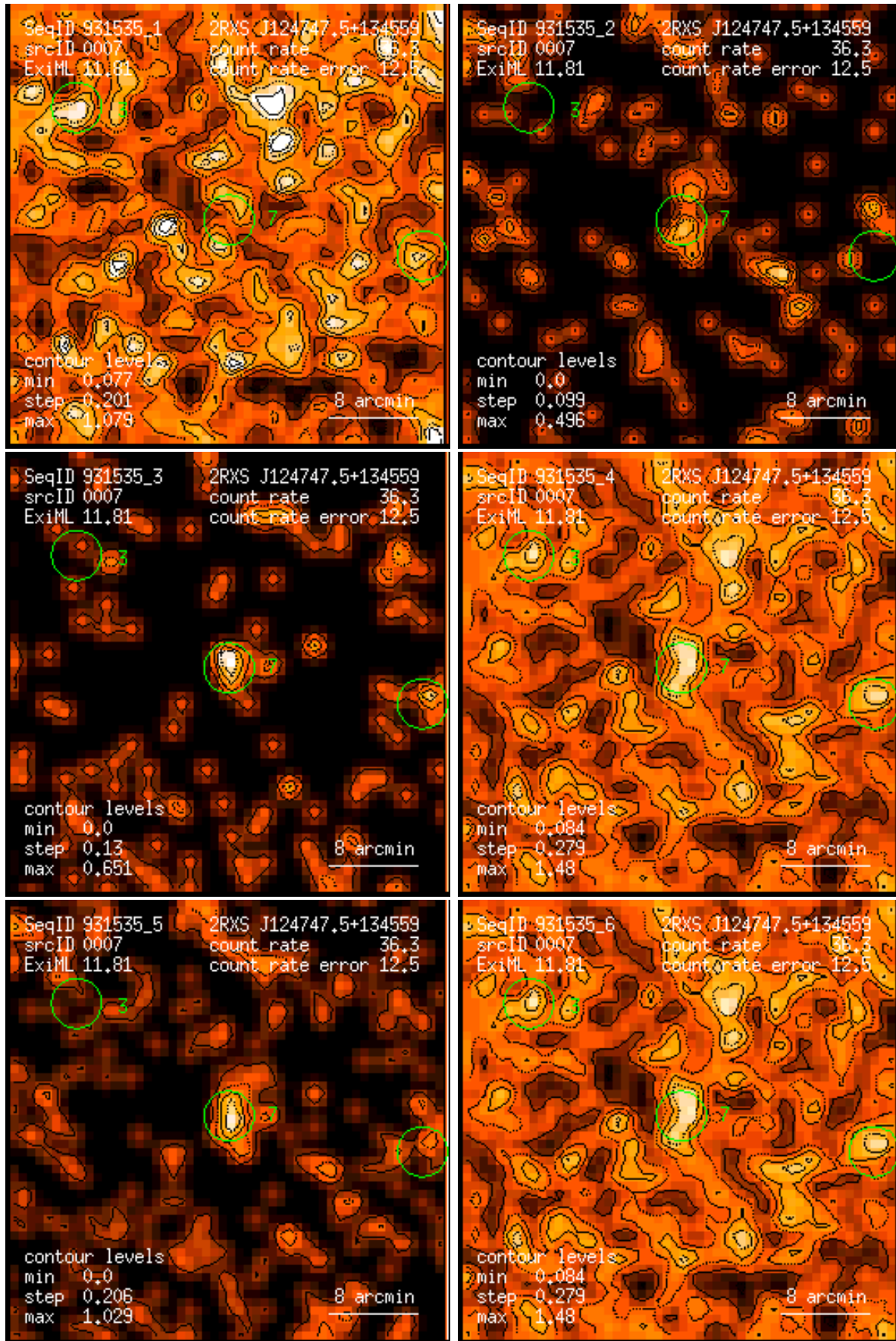
Figure 7: RASS 931535: detection 0007: band rate images, Gaussian filter: (1) PSPC channels 11 – 41, (2) 52 – 90, (3) 91 – 201, (4) 11 – 235, (5) 52 – 201, (6) 11 – 201. Broad band rates in counts/ks. Band rate contour levels in counts/ks/arcmin 2 .
