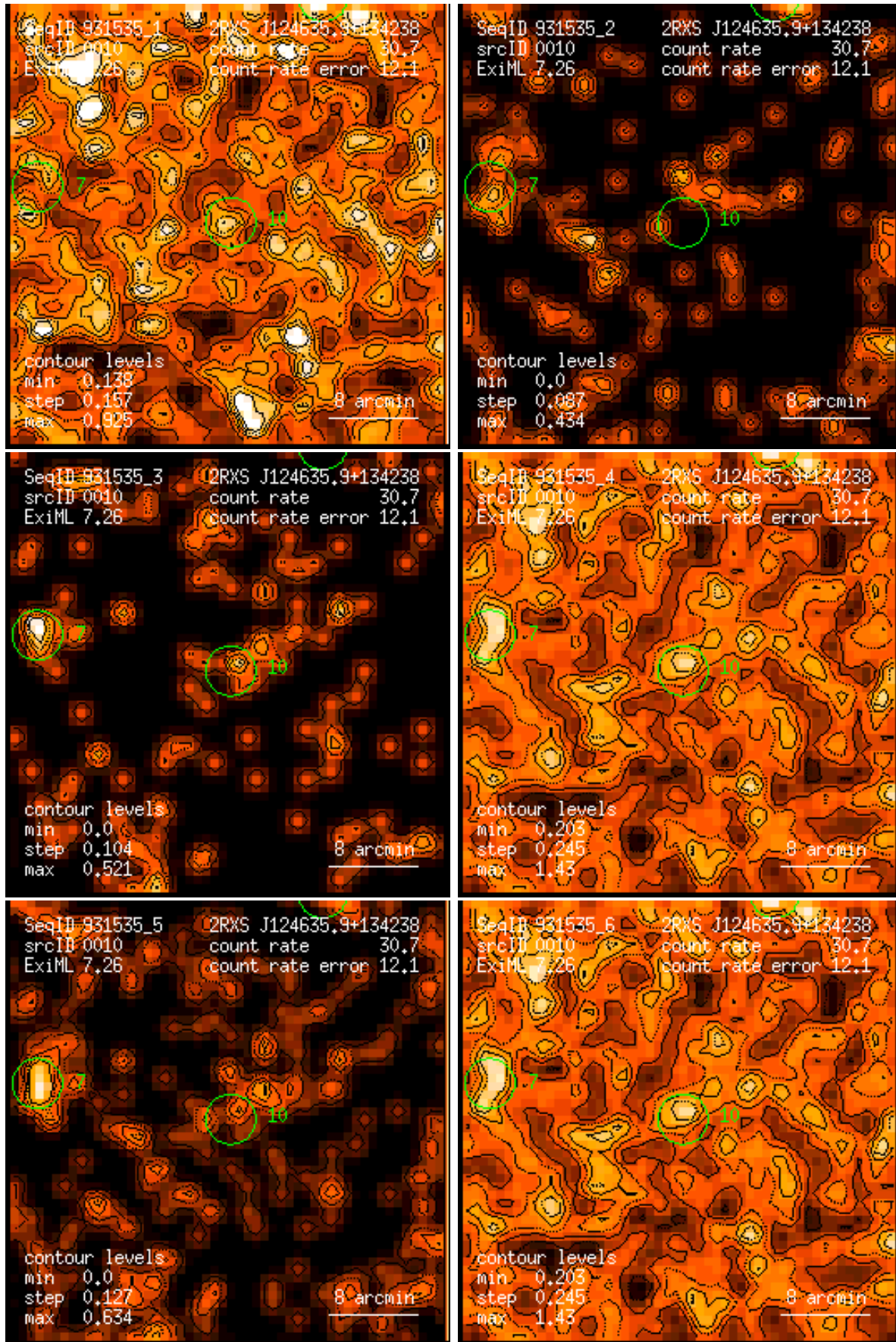
Figure 10: RASS 931535: detection 0010: band rate images, Gaussian filter: (1) PSPC channels 11 – 41, (2) 52 – 90, (3) 91 – 201, (4) 11 – 235, (5) 52 – 201, (6) 11 – 201. Broad band rates in counts/ks. Band rate contour levels in counts/ks/arcmin 2 .
