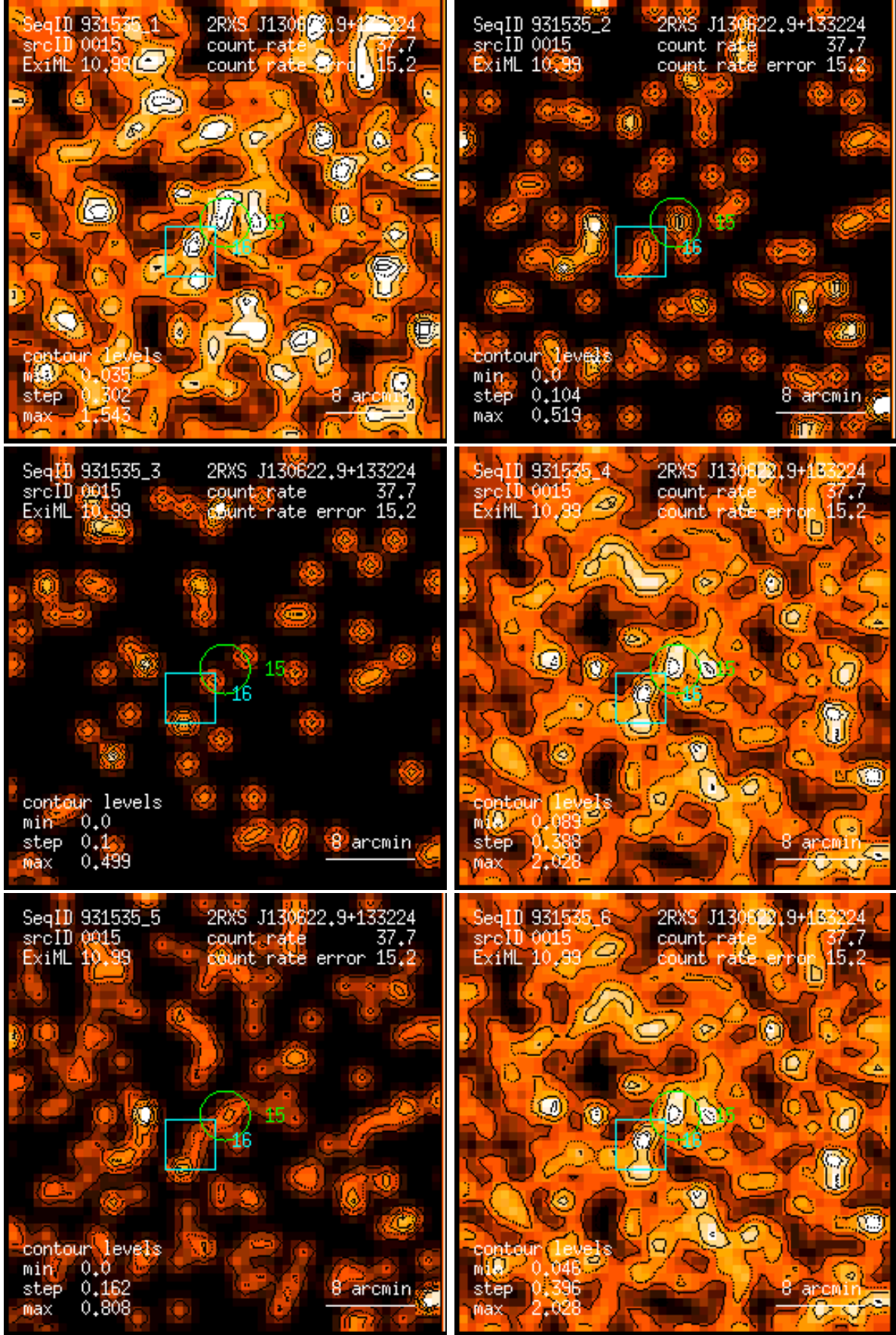
Figure 15: RASS 931535: detection 0015: band rate images, Gaussian filter: (1) PSPC channels 11 – 41, (2) 52 – 90, (3) 91 – 201, (4) 11 – 235, (5) 52 – 201, (6) 11 – 201. Broad band rates in counts/ks. Band rate contour levels in counts/ks/arcmin 2 .
