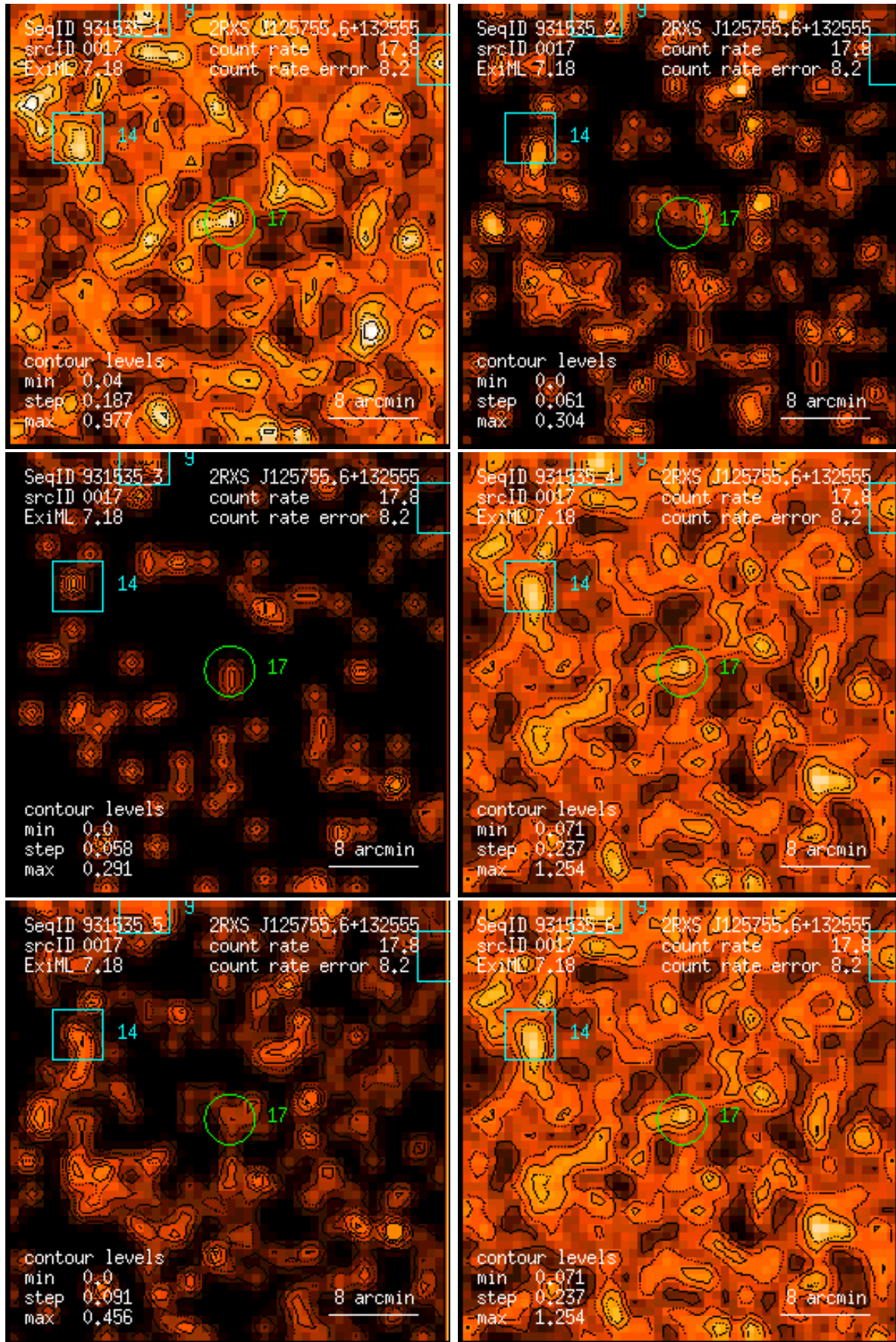
Figure 17: RASS 931535: detection 0017: band rate images, Gaussian filter: (1) PSPC channels 11 – 41, (2) 52 – 90, (3) 91 – 201, (4) 11 – 235, (5) 52 – 201, (6) 11 – 201. Broad band rates in counts/ks. Band rate contour levels in counts/ks/arcmin 2 .
