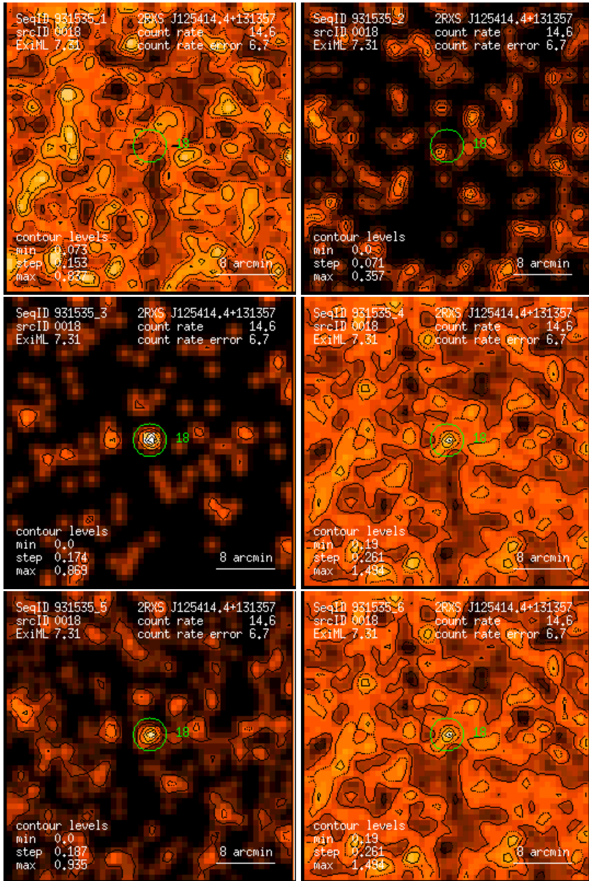
Figure 18: RASS 931535: detection 0018: band rate images, Gaussian filter: (1) PSPC channels 11 – 41, (2) 52 – 90, (3) 91 – 201, (4) 11 – 235, (5) 52 – 201, (6) 11 – 201. Broad band rates in counts/ks. Band rate contour levels in counts/ks/arcmin 2 .
