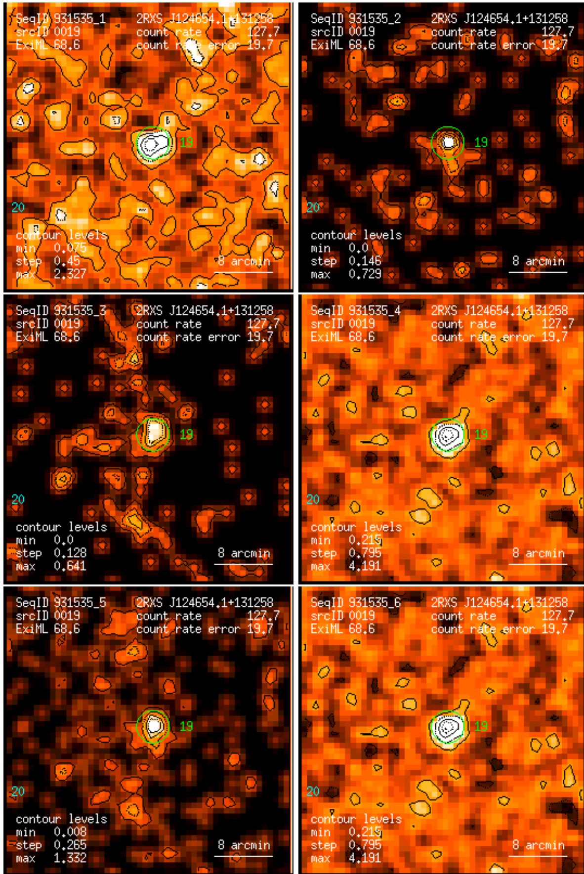
Figure 19: RASS 931535: detection 0019: band rate images, Gaussian filter: (1) PSPC channels 11 – 41, (2) 52 – 90, (3) 91 – 201, (4) 11 – 235, (5) 52 – 201, (6) 11 – 201. Broad band rates in counts/ks. Band rate contour levels in counts/ks/arcmin 2 .
