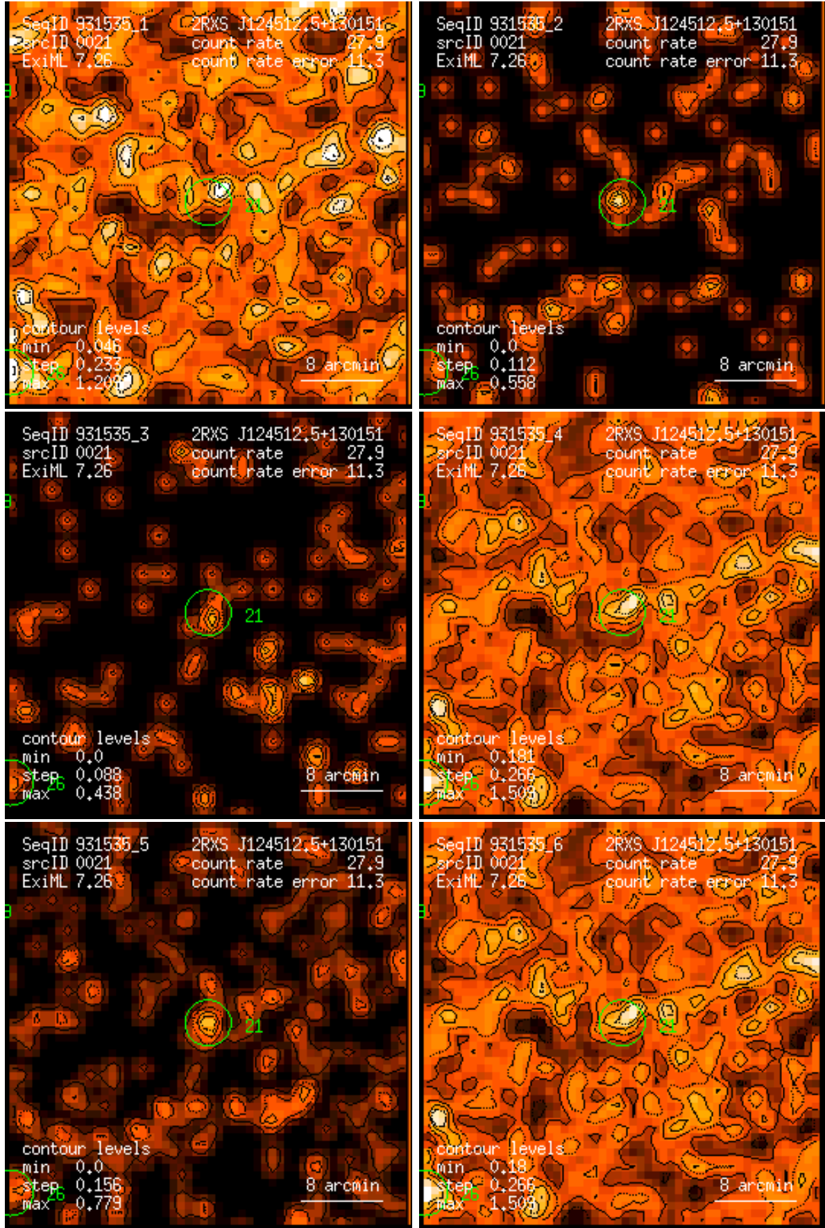
Figure 21: RASS 931535: detection 0021: band rate images, Gaussian filter: (1) PSPC channels 11 – 41, (2) 52 – 90, (3) 91 – 201, (4) 11 – 235, (5) 52 – 201, (6) 11 – 201. Broad band rates in counts/ks. Band rate contour levels in counts/ks/arcmin 2 .
