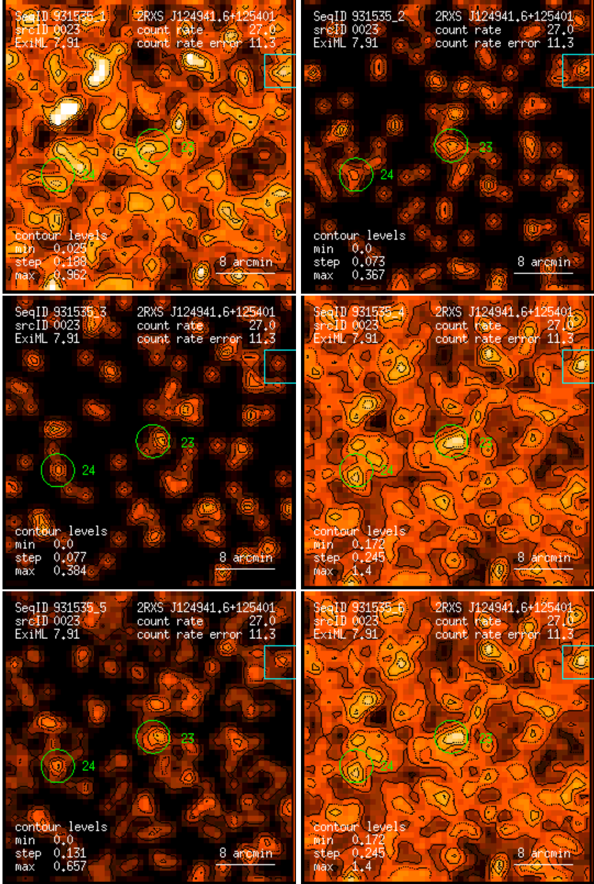
Figure 23: RASS 931535: detection 0023: band rate images, Gaussian filter: (1) PSPC channels 11 – 41, (2) 52 – 90, (3) 91 – 201, (4) 11 – 235, (5) 52 – 201, (6) 11 – 201. Broad band rates in counts/ks. Band rate contour levels in counts/ks/arcmin 2 .
