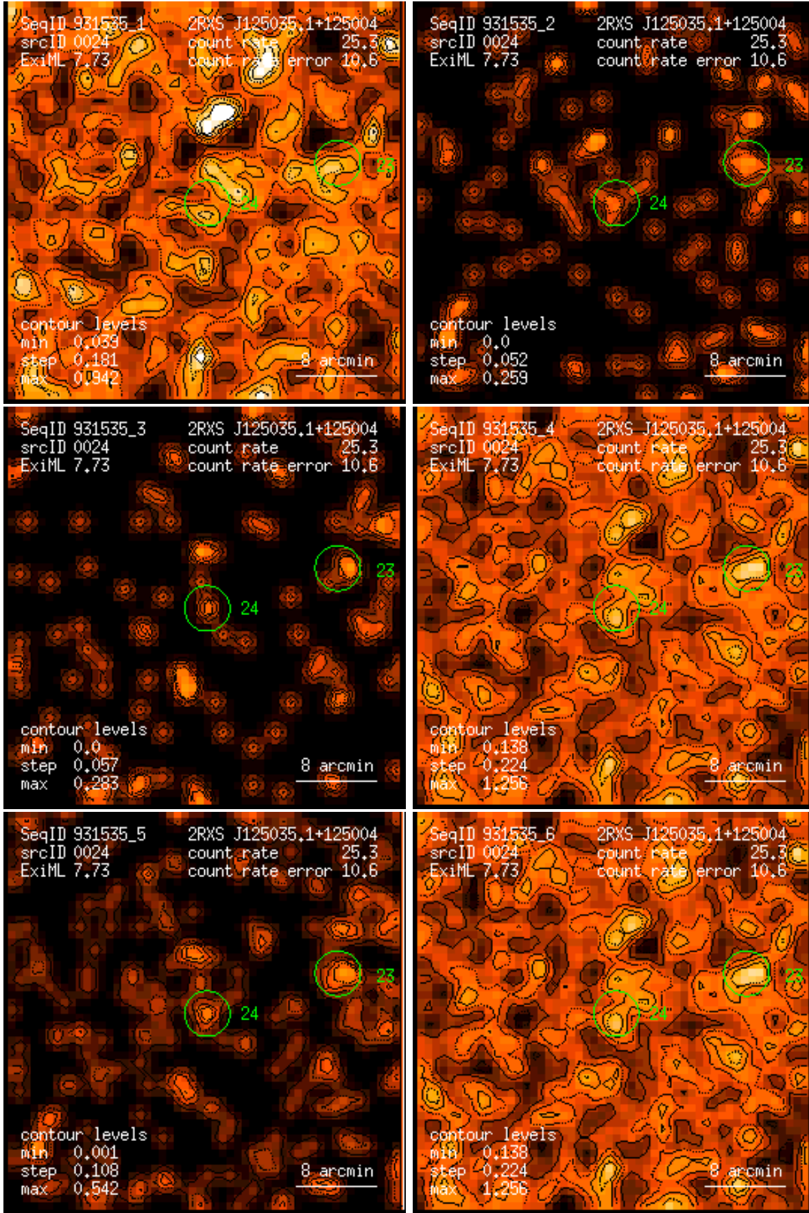
Figure 24: RASS 931535: detection 0024: band rate images, Gaussian filter: (1) PSPC channels 11 – 41, (2) 52 – 90, (3) 91 – 201, (4) 11 – 235, (5) 52 – 201, (6) 11 – 201. Broad band rates in counts/ks. Band rate contour levels in counts/ks/arcmin 2 .
