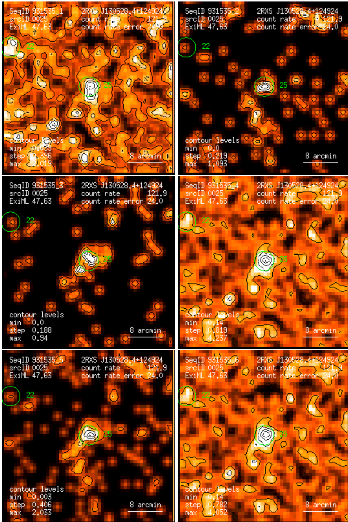
Figure 25: RASS 931535: detection 0025: band rate images, Gaussian filter: (1) PSPC channels 11 – 41, (2) 52 – 90, (3) 91 – 201, (4) 11 – 235, (5) 52 – 201, (6) 11 – 201. Broad band rates in counts/ks. Band rate contour levels in counts/ks/arcmin 2 .
