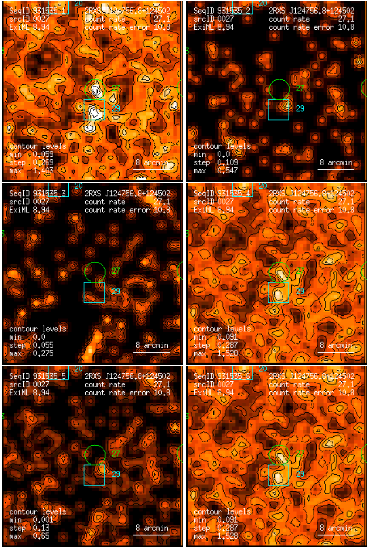
Figure 27: RASS 931535: detection 0027: band rate images, Gaussian filter: (1) PSPC channels 11 – 41, (2) 52 – 90, (3) 91 – 201, (4) 11 – 235, (5) 52 – 201, (6) 11 – 201. Broad band rates in counts/ks. Band rate contour levels in counts/ks/arcmin 2 .
