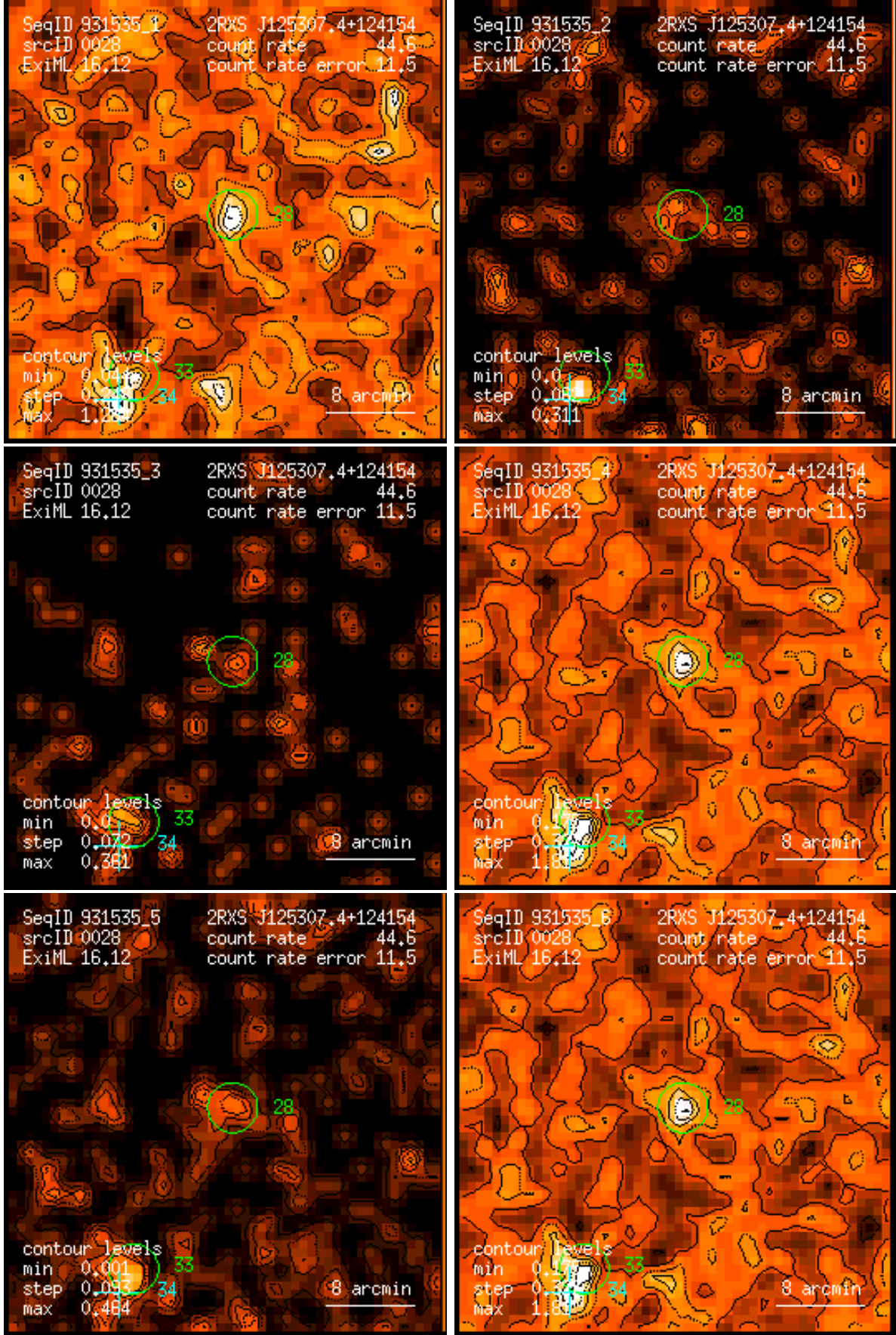
Figure 28: RASS 931535: detection 0028: band rate images, Gaussian filter: (1) PSPC channels 11 – 41, (2) 52 – 90, (3) 91 – 201, (4) 11 – 235, (5) 52 – 201, (6) 11 – 201. Broad band rates in counts/ks. Band rate contour levels in counts/ks/arcmin 2 .
