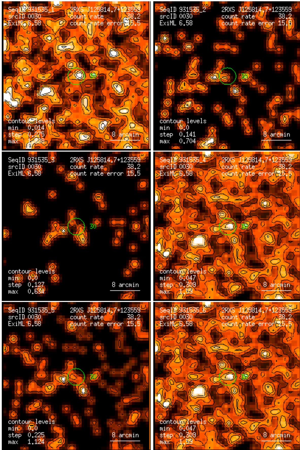
Figure 30: RASS 931535: detection 0030: band rate images, Gaussian filter: (1) PSPC channels 11 – 41, (2) 52 – 90, (3) 91 – 201, (4) 11 – 235, (5) 52 – 201, (6) 11 – 201. Broad band rates in counts/ks. Band rate contour levels in counts/ks/arcmin 2 .
