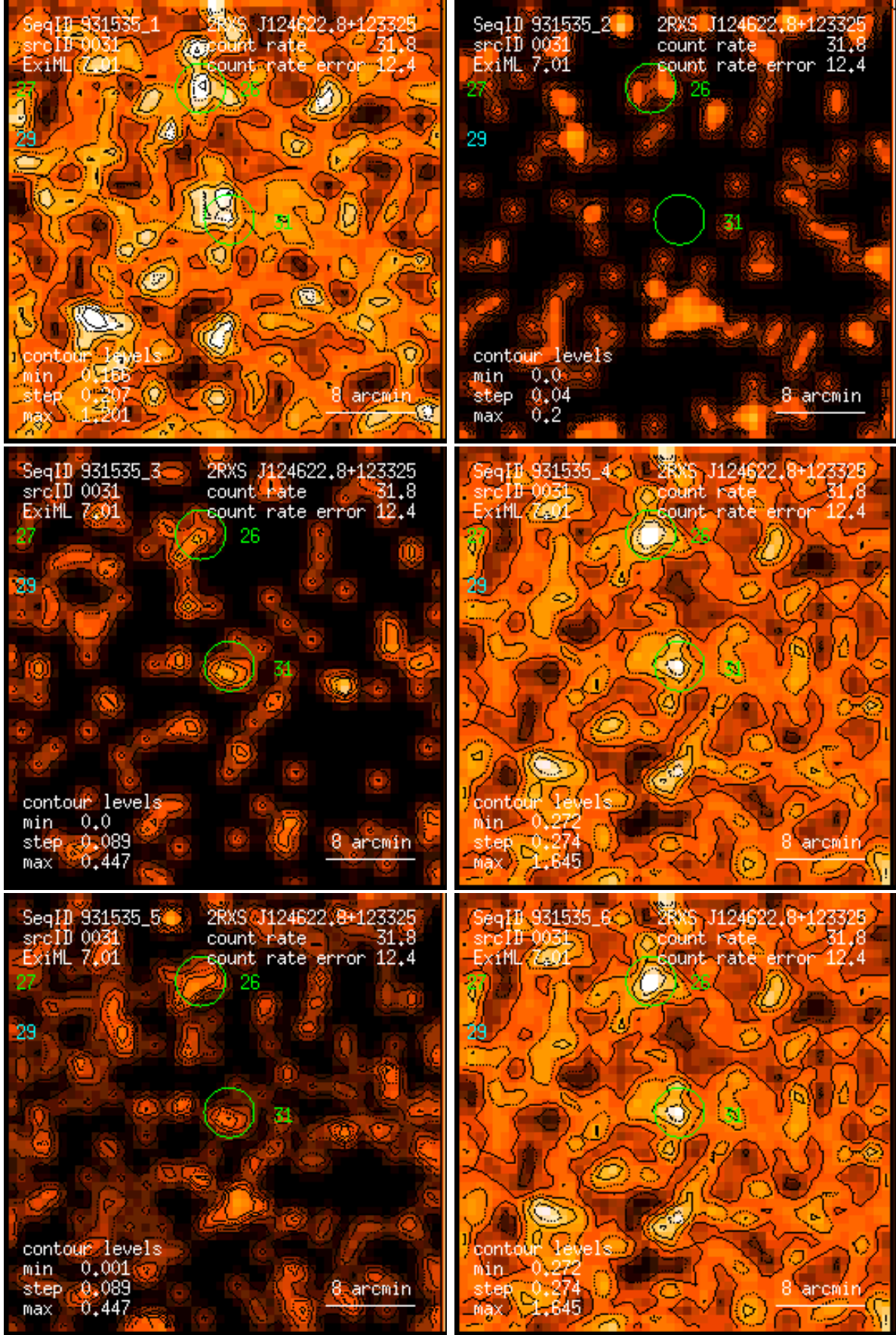
Figure 31: RASS 931535: detection 0031: band rate images, Gaussian filter: (1) PSPC channels 11 – 41, (2) 52 – 90, (3) 91 – 201, (4) 11 – 235, (5) 52 – 201, (6) 11 – 201. Broad band rates in counts/ks. Band rate contour levels in counts/ks/arcmin 2 .
