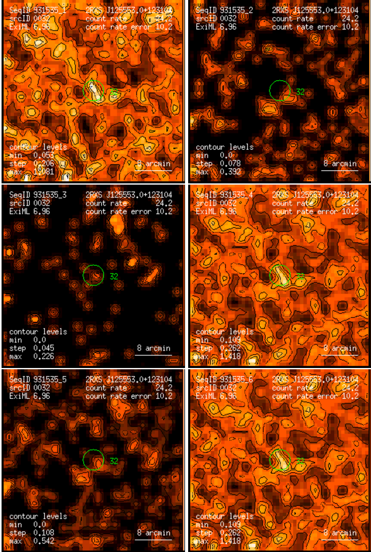
Figure 32: RASS 931535: detection 0032: band rate images, Gaussian filter: (1) PSPC channels 11 – 41, (2) 52 – 90, (3) 91 – 201, (4) 11 – 235, (5) 52 – 201, (6) 11 – 201. Broad band rates in counts/ks. Band rate contour levels in counts/ks/arcmin 2 .
