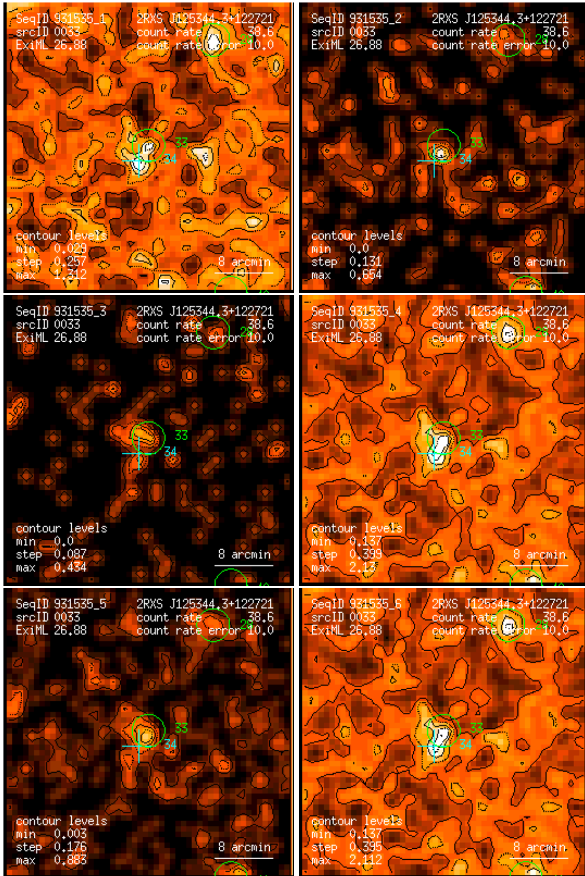
Figure 33: RASS 931535: detection 0033: band rate images, Gaussian filter: (1) PSPC channels 11 – 41, (2) 52 – 90, (3) 91 – 201, (4) 11 – 235, (5) 52 – 201, (6) 11 – 201. Broad band rates in counts/ks. Band rate contour levels in counts/ks/arcmin 2 .
