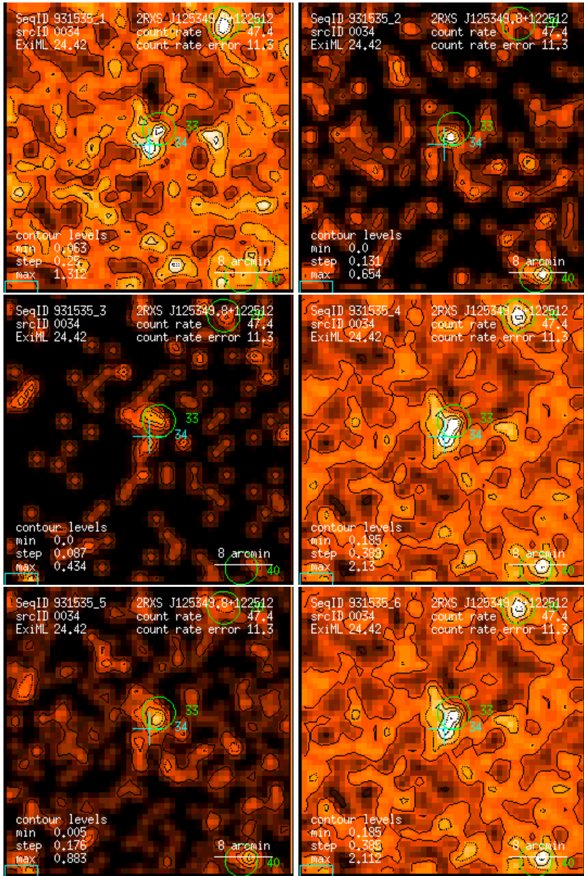
Figure 34: RASS 931535: detection 0034: band rate images, Gaussian filter: (1) PSPC channels 11 – 41, (2) 52 – 90, (3) 91 – 201, (4) 11 – 235, (5) 52 – 201, (6) 11 – 201. Broad band rates in counts/ks. Band rate contour levels in counts/ks/arcmin 2 .
