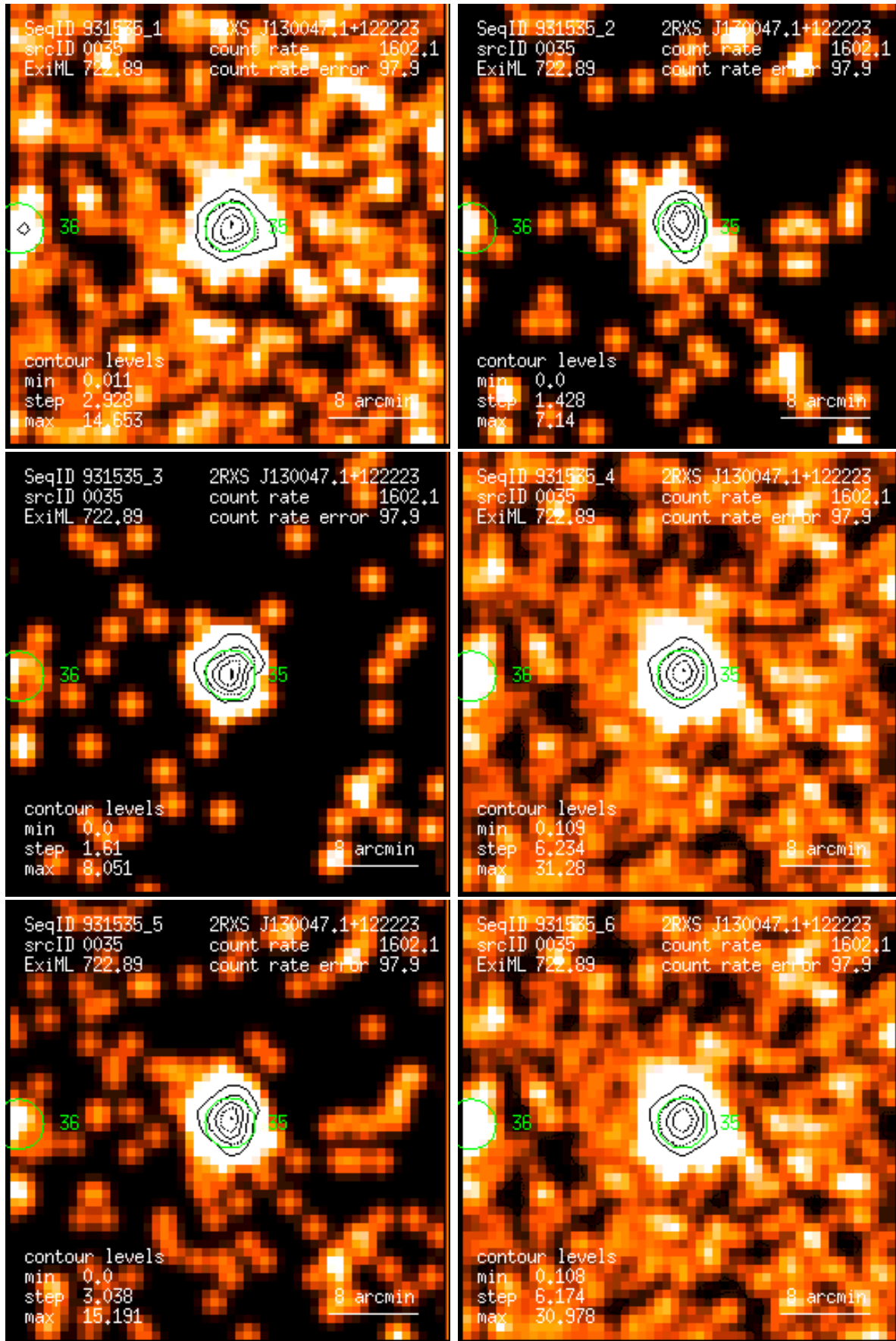
Figure 35: RASS 931535: detection 0035: band rate images, Gaussian filter: (1) PSPC channels 11 – 41, (2) 52 – 90, (3) 91 – 201, (4) 11 – 235, (5) 52 – 201, (6) 11 – 201. Broad band rates in counts/ks. Band rate contour levels in counts/ks/arcmin 2 .
