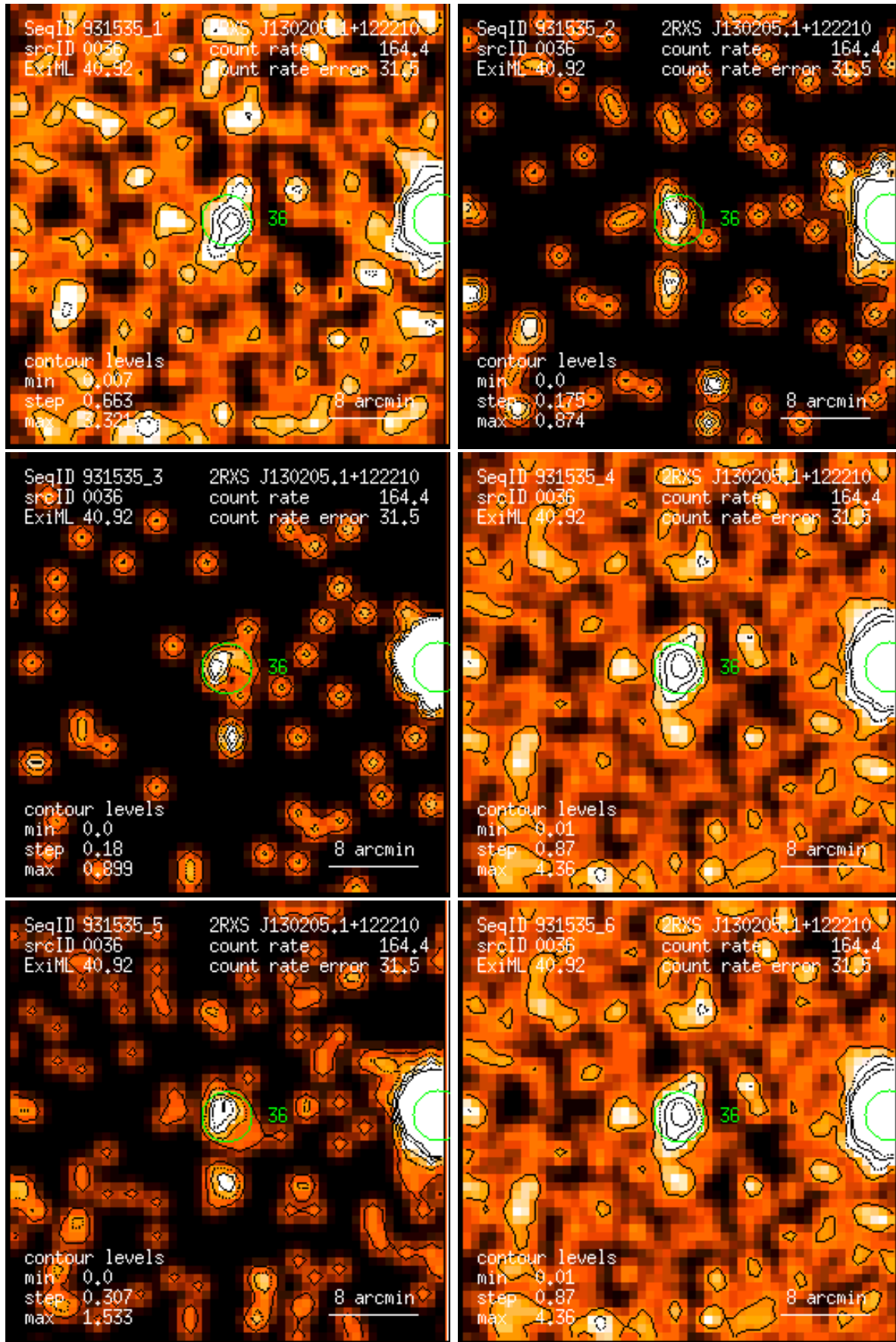
Figure 36: RASS 931535: detection 0036: band rate images, Gaussian filter: (1) PSPC channels 11 – 41, (2) 52 – 90, (3) 91 – 201, (4) 11 – 235, (5) 52 – 201, (6) 11 – 201. Broad band rates in counts/ks. Band rate contour levels in counts/ks/arcmin 2 .
