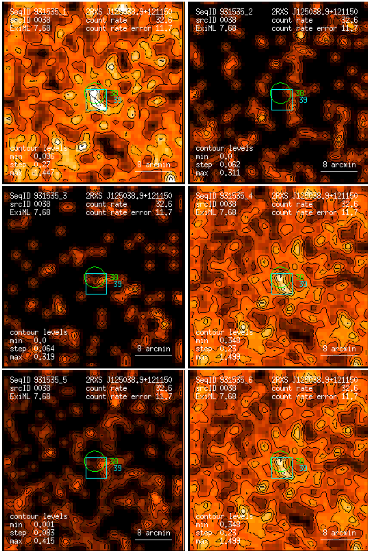
Figure 38: RASS 931535: detection 0038: band rate images, Gaussian filter: (1) PSPC channels 11 – 41, (2) 52 – 90, (3) 91 – 201, (4) 11 – 235, (5) 52 – 201, (6) 11 – 201. Broad band rates in counts/ks. Band rate contour levels in counts/ks/arcmin 2 .
