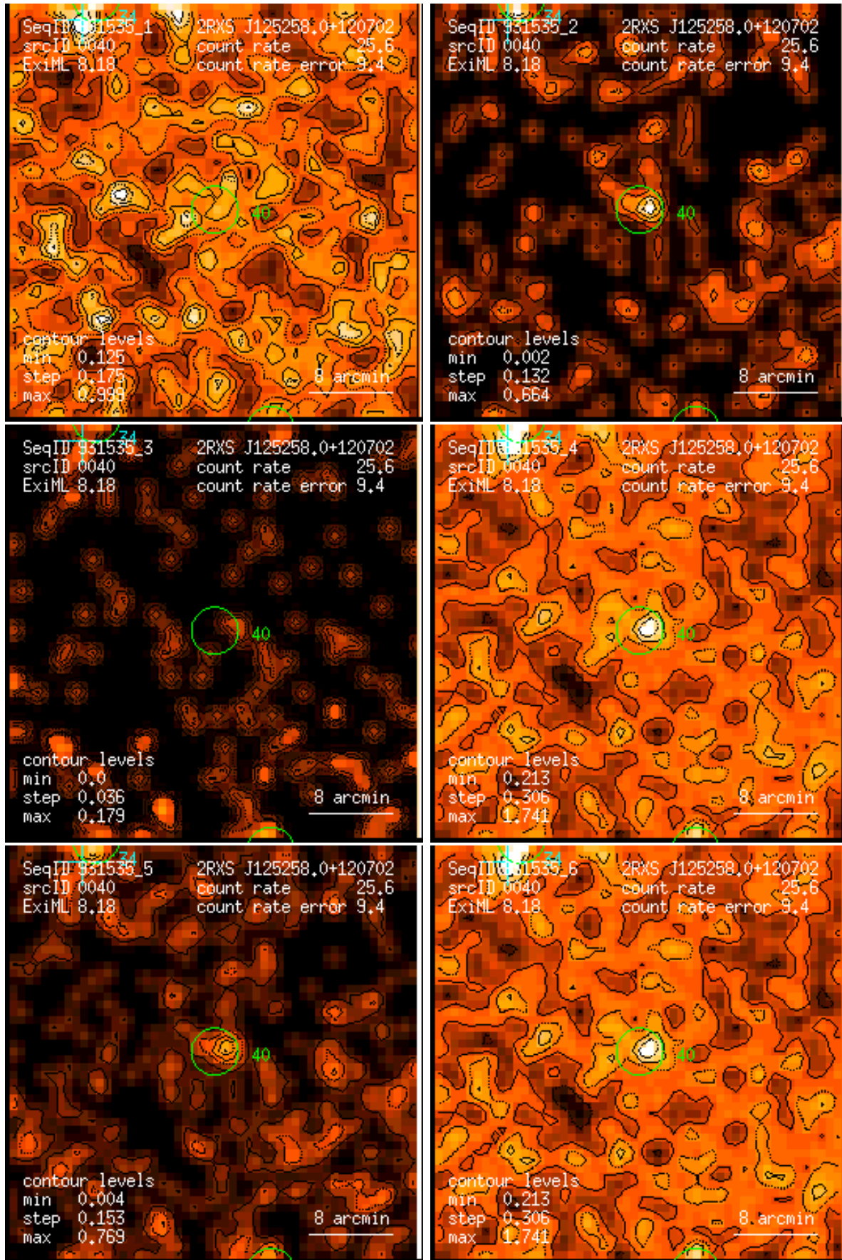
Figure 40: RASS 931535: detection 0040: band rate images, Gaussian filter: (1) PSPC channels 11 – 41, (2) 52 – 90, (3) 91 – 201, (4) 11 – 235, (5) 52 – 201, (6) 11 – 201. Broad band rates in counts/ks. Band rate contour levels in counts/ks/arcmin 2 .
