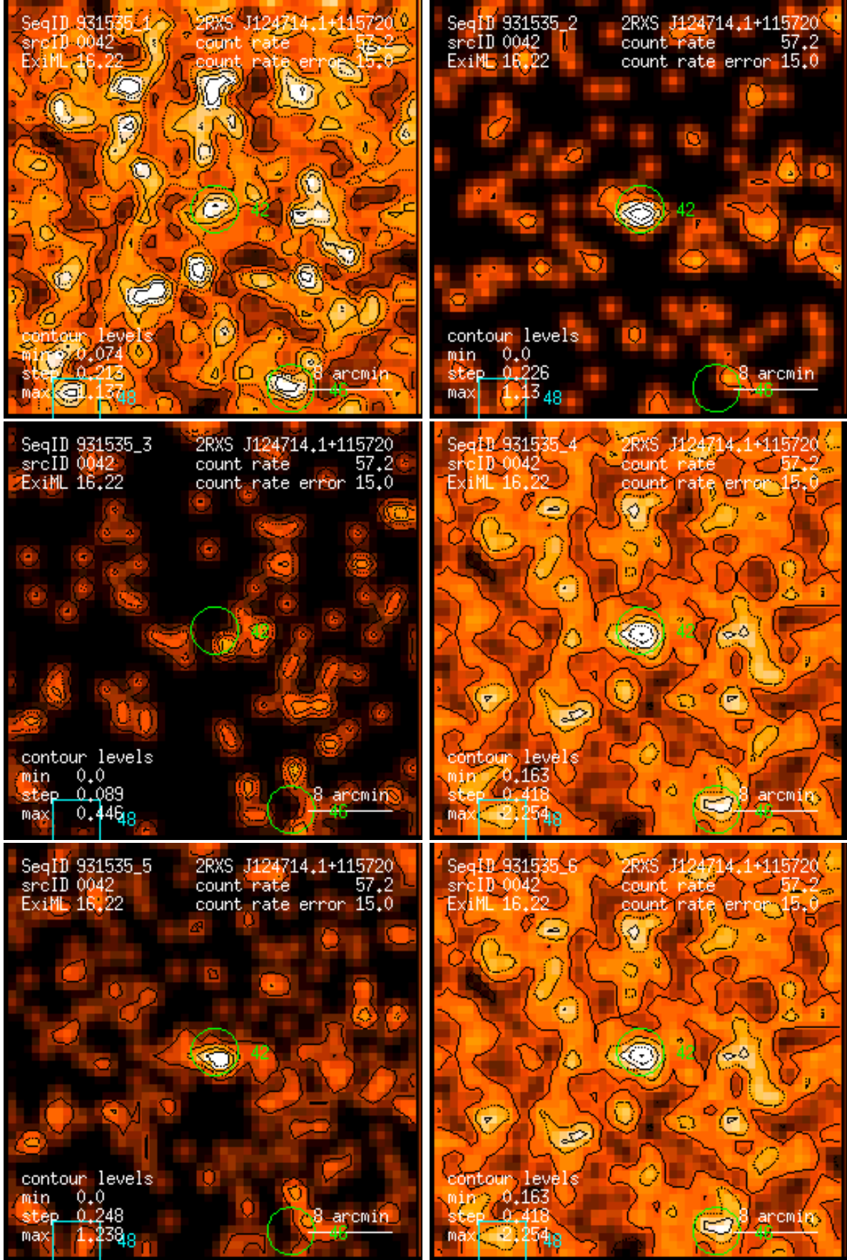
Figure 42: RASS 931535: detection 0042: band rate images, Gaussian filter: (1) PSPC channels 11 – 41, (2) 52 – 90, (3) 91 – 201, (4) 11 – 235, (5) 52 – 201, (6) 11 – 201. Broad band rates in counts/ks. Band rate contour levels in counts/ks/arcmin 2 .
