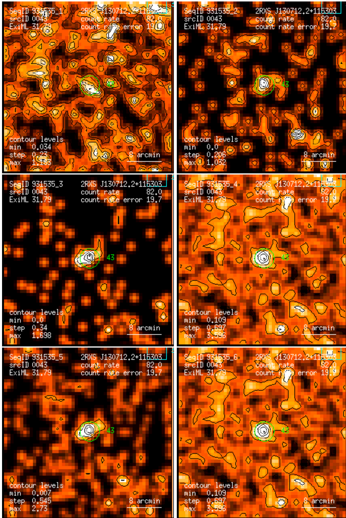
Figure 43: RASS 931535: detection 0043: band rate images, Gaussian filter: (1) PSPC channels 11 – 41, (2) 52 – 90, (3) 91 – 201, (4) 11 – 235, (5) 52 – 201, (6) 11 – 201. Broad band rates in counts/ks. Band rate contour levels in counts/ks/arcmin 2 .
