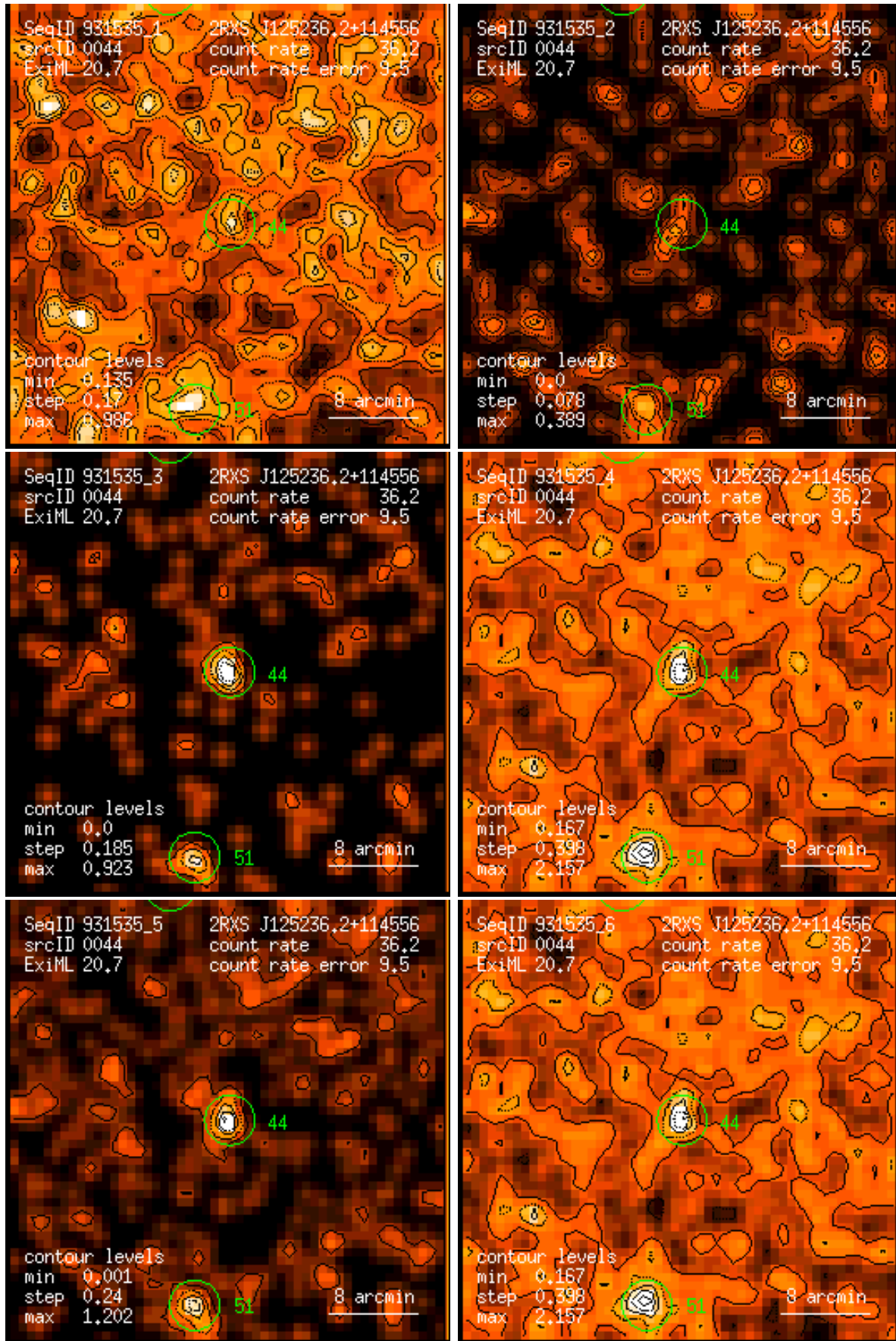
Figure 44: RASS 931535: detection 0044: band rate images, Gaussian filter: (1) PSPC channels 11 – 41, (2) 52 – 90, (3) 91 – 201, (4) 11 – 235, (5) 52 – 201, (6) 11 – 201. Broad band rates in counts/ks. Band rate contour levels in counts/ks/arcmin 2 .
