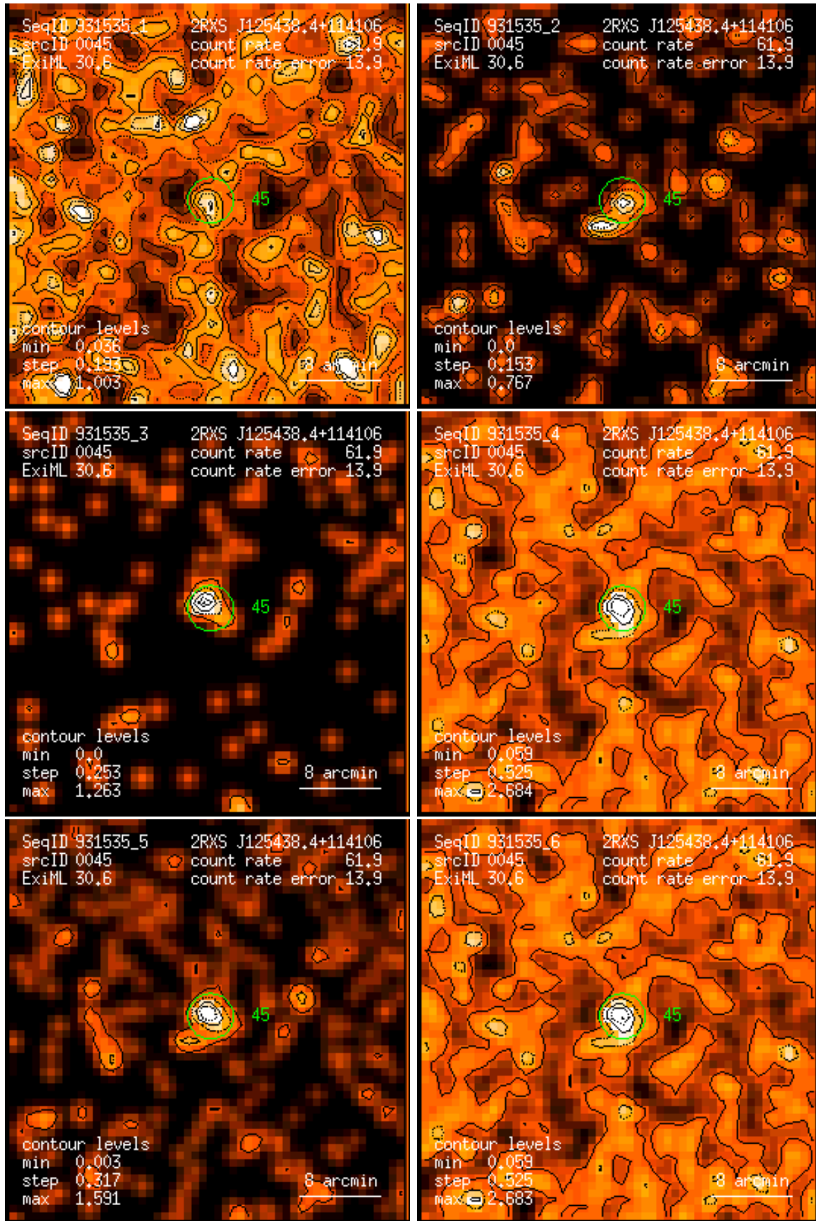
Figure 45: RASS 931535: detection 0045: band rate images, Gaussian filter: (1) PSPC channels 11 – 41, (2) 52 – 90, (3) 91 – 201, (4) 11 – 235, (5) 52 – 201, (6) 11 – 201. Broad band rates in counts/ks. Band rate contour levels in counts/ks/arcmin 2 .
