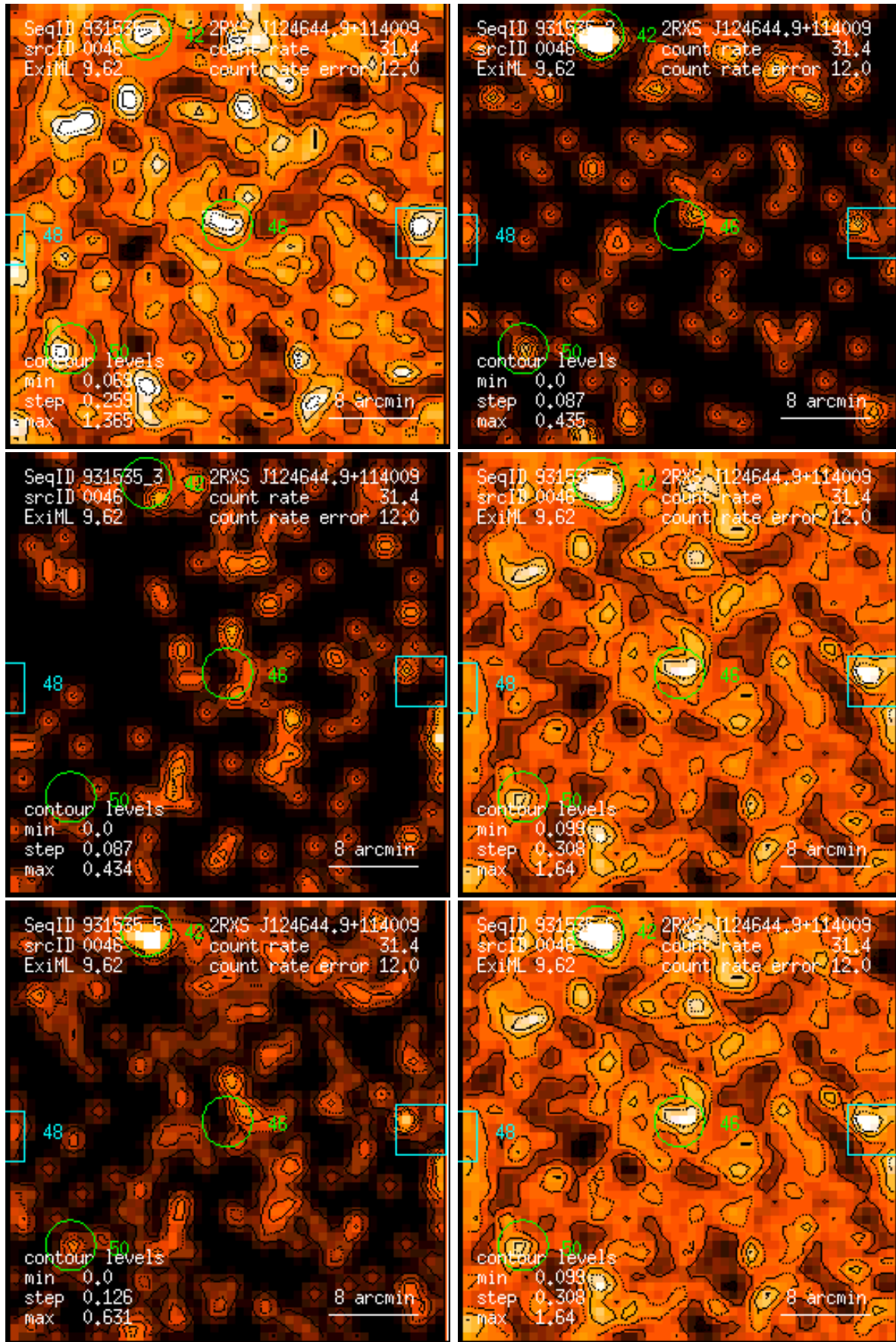
Figure 46: RASS 931535: detection 0046: band rate images, Gaussian filter: (1) PSPC channels 11 – 41, (2) 52 – 90, (3) 91 – 201, (4) 11 – 235, (5) 52 – 201, (6) 11 – 201. Broad band rates in counts/ks. Band rate contour levels in counts/ks/arcmin 2 .
