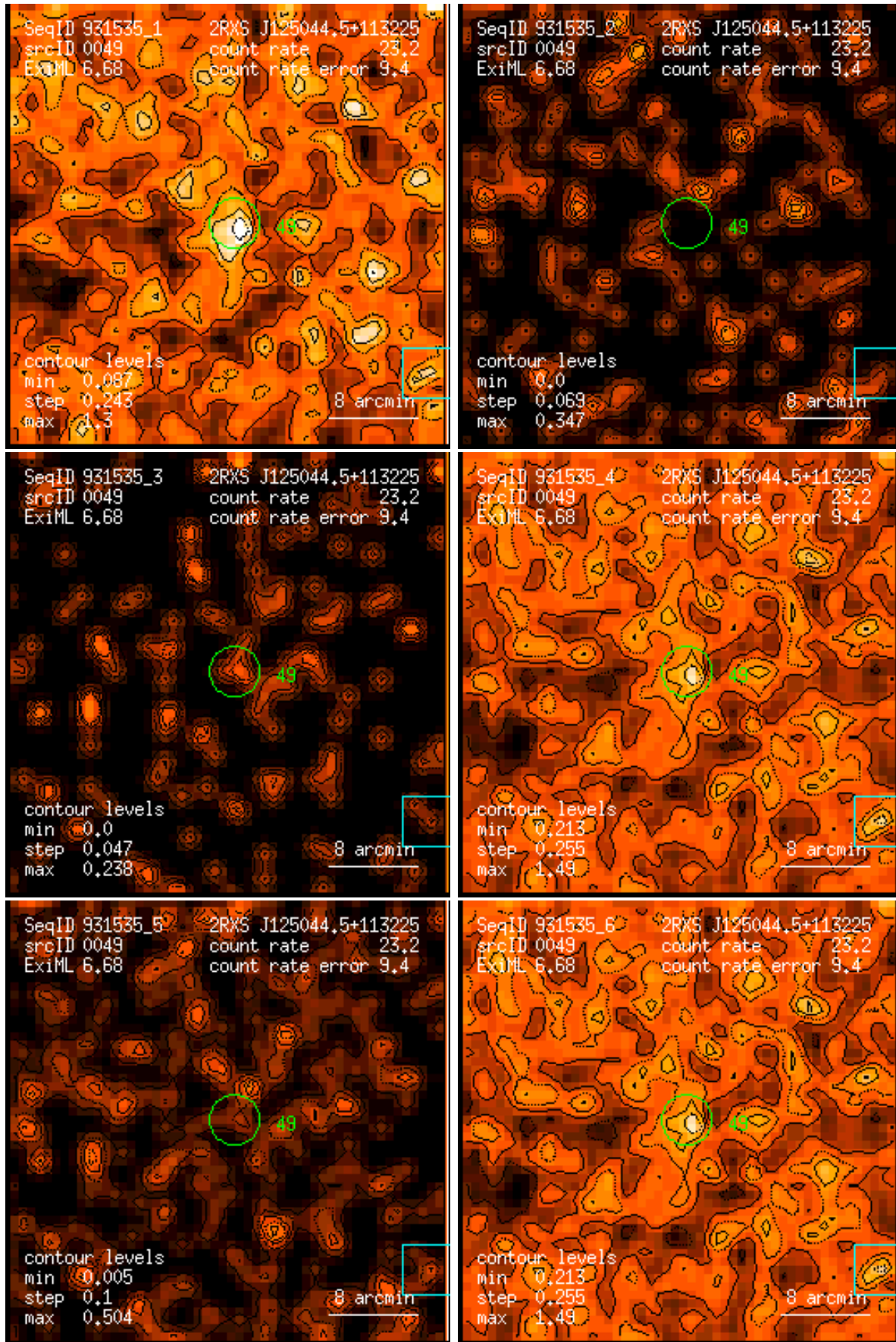
Figure 49: RASS 931535: detection 0049: band rate images, Gaussian filter: (1) PSPC channels 11 – 41, (2) 52 – 90, (3) 91 – 201, (4) 11 – 235, (5) 52 – 201, (6) 11 – 201. Broad band rates in counts/ks. Band rate contour levels in counts/ks/arcmin 2 .
