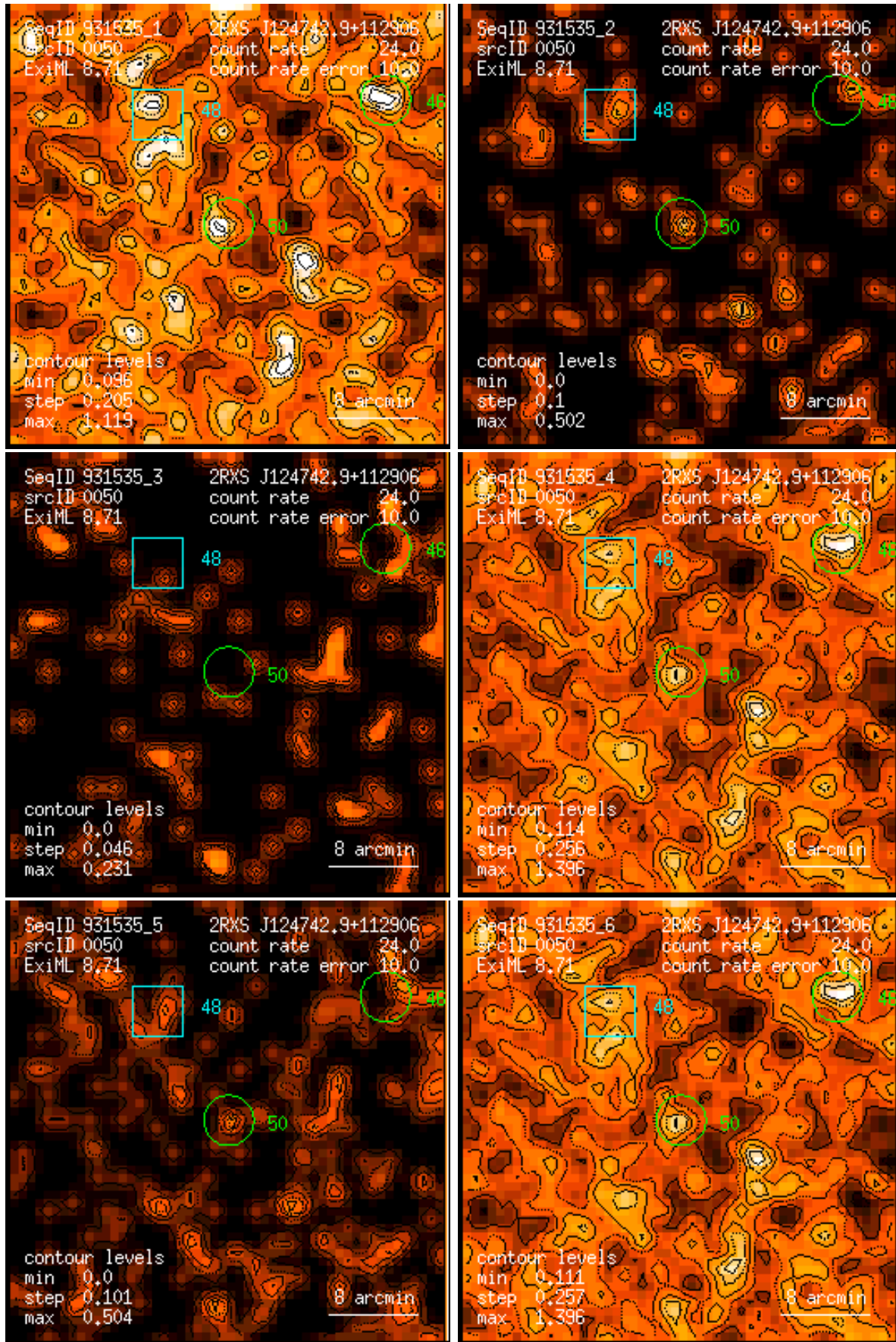
Figure 50: RASS 931535: detection 0050: band rate images, Gaussian filter: (1) PSPC channels 11 – 41, (2) 52 – 90, (3) 91 – 201, (4) 11 – 235, (5) 52 – 201, (6) 11 – 201. Broad band rates in counts/ks. Band rate contour levels in counts/ks/arcmin 2 .
