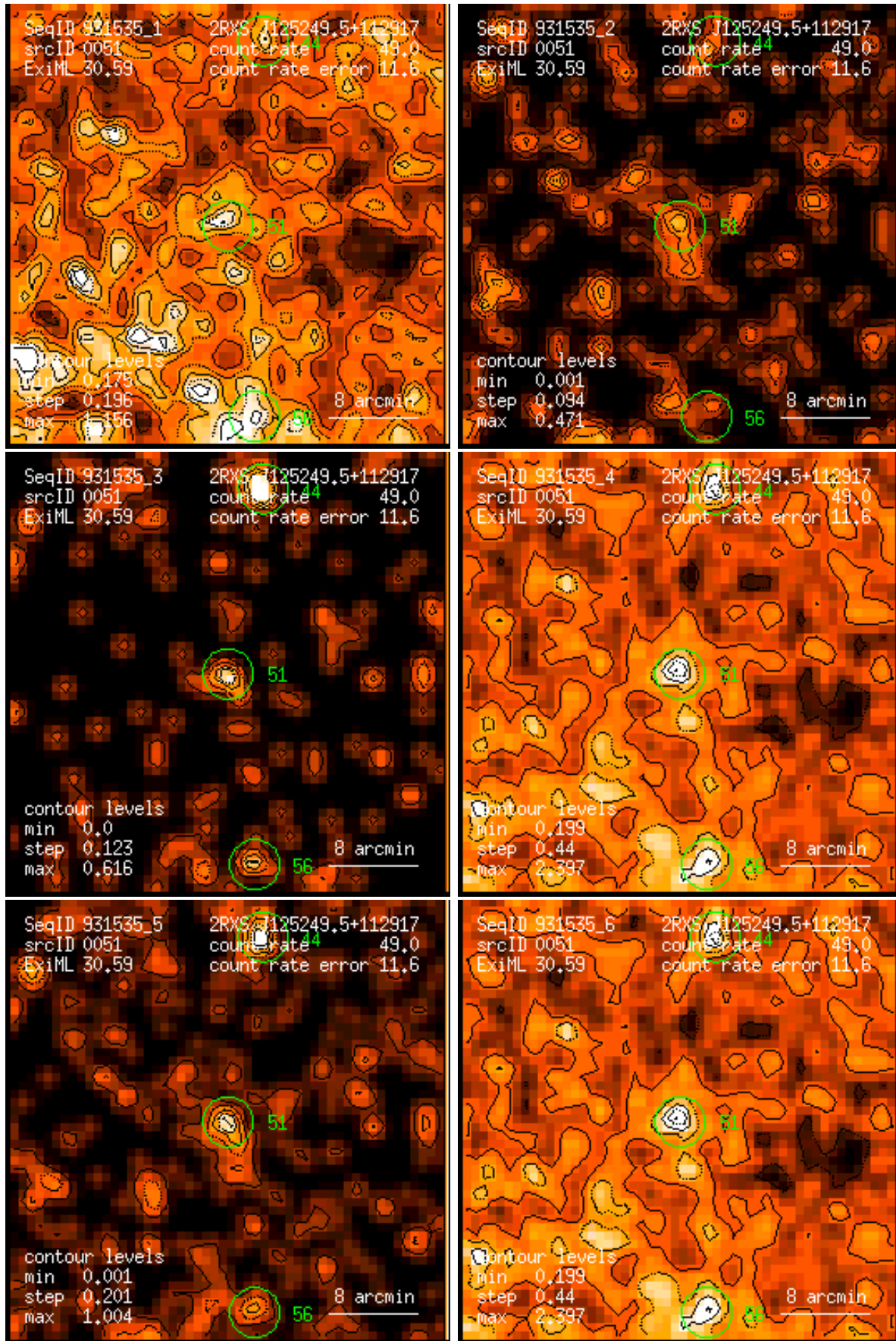
Figure 51: RASS 931535: detection 0051: band rate images, Gaussian filter: (1) PSPC channels 11 – 41, (2) 52 – 90, (3) 91 – 201, (4) 11 – 235, (5) 52 – 201, (6) 11 – 201. Broad band rates in counts/ks. Band rate contour levels in counts/ks/arcmin 2 .
