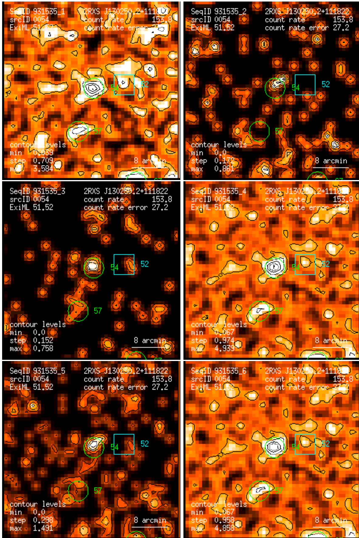
Figure 54: RASS 931535: detection 0054: band rate images, Gaussian filter: (1) PSPC channels 11 – 41, (2) 52 – 90, (3) 91 – 201, (4) 11 – 235, (5) 52 – 201, (6) 11 – 201. Broad band rates in counts/ks. Band rate contour levels in counts/ks/arcmin 2 .
