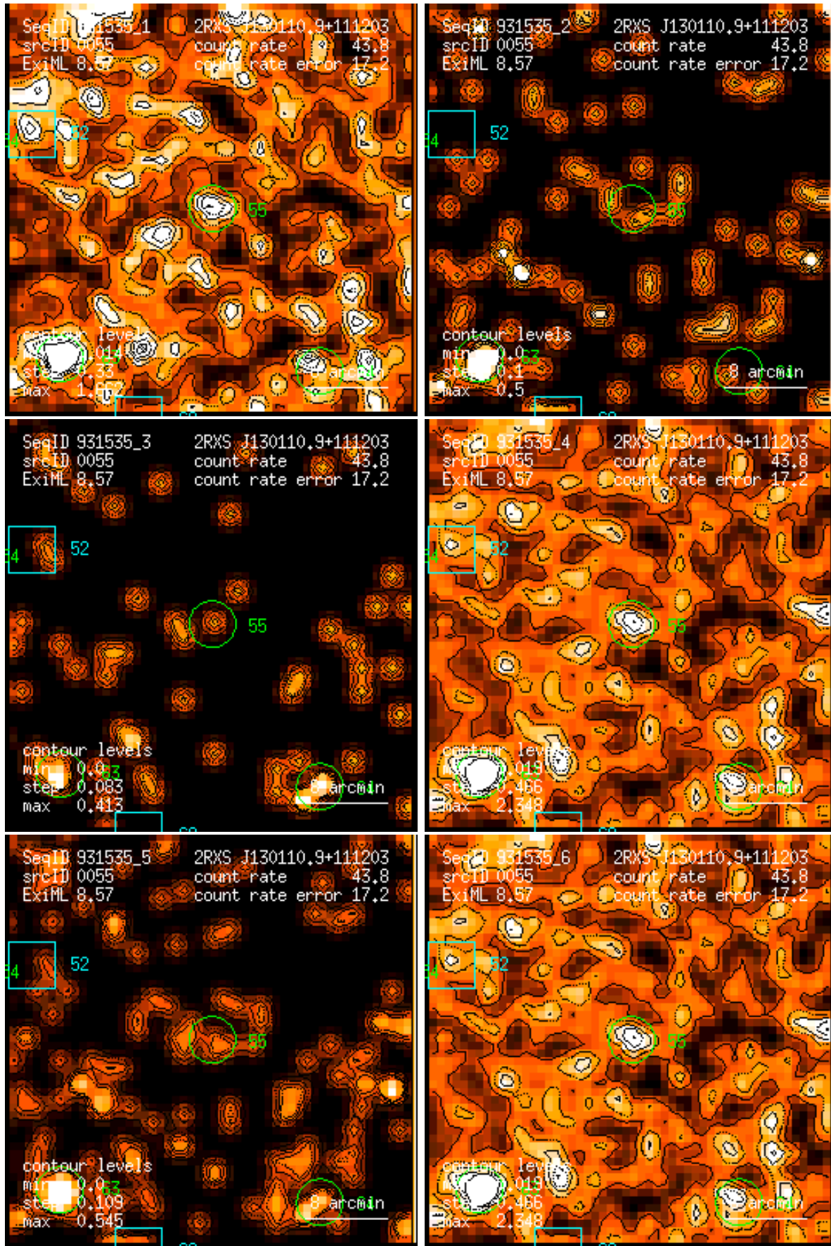
Figure 55: RASS 931535: detection 0055: band rate images, Gaussian filter: (1) PSPC channels 11 – 41, (2) 52 – 90, (3) 91 – 201, (4) 11 – 235, (5) 52 – 201, (6) 11 – 201. Broad band rates in counts/ks. Band rate contour levels in counts/ks/arcmin 2 .
