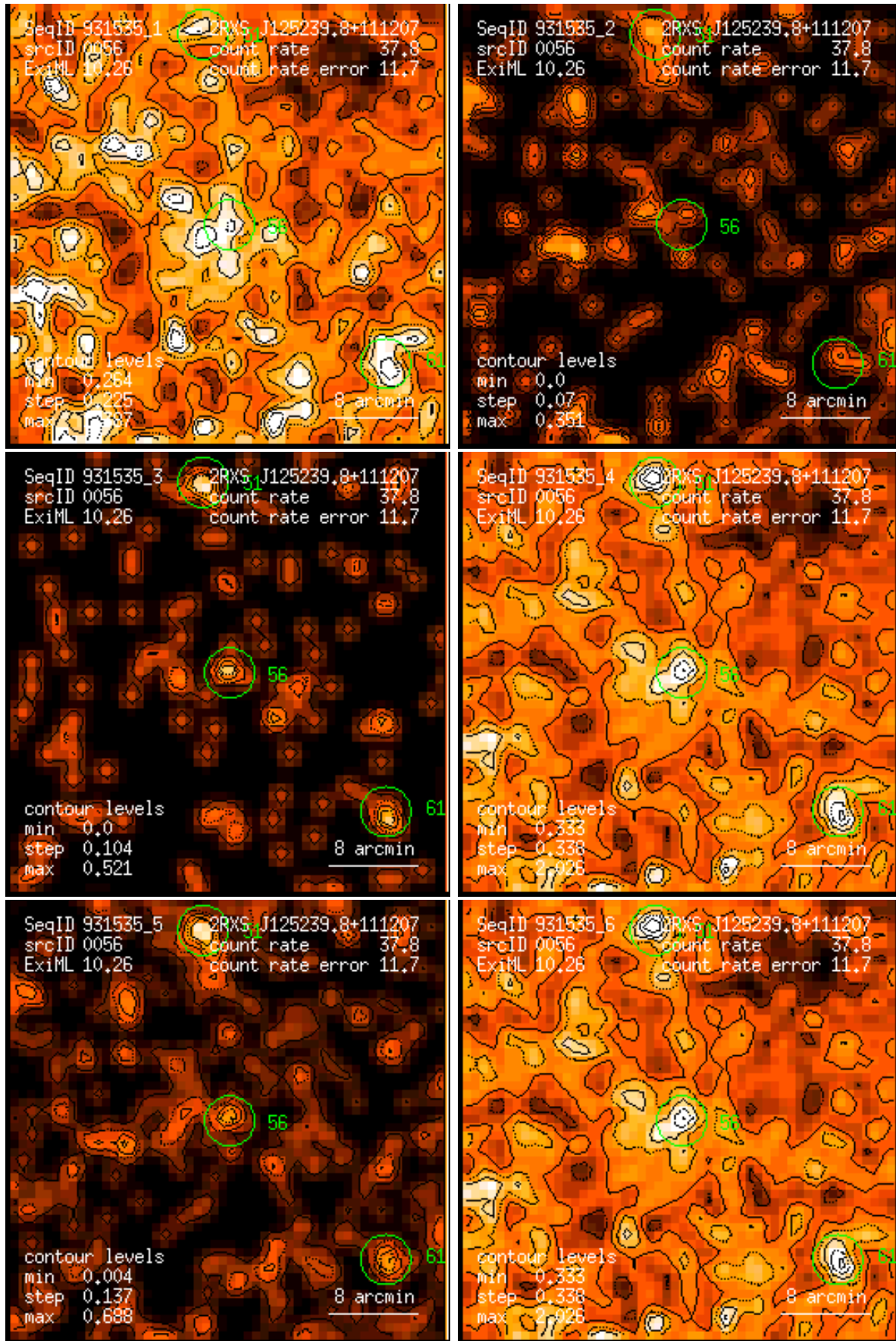
Figure 56: RASS 931535: detection 0056: band rate images, Gaussian filter: (1) PSPC channels 11 – 41, (2) 52 – 90, (3) 91 – 201, (4) 11 – 235, (5) 52 – 201, (6) 11 – 201. Broad band rates in counts/ks. Band rate contour levels in counts/ks/arcmin 2 .
