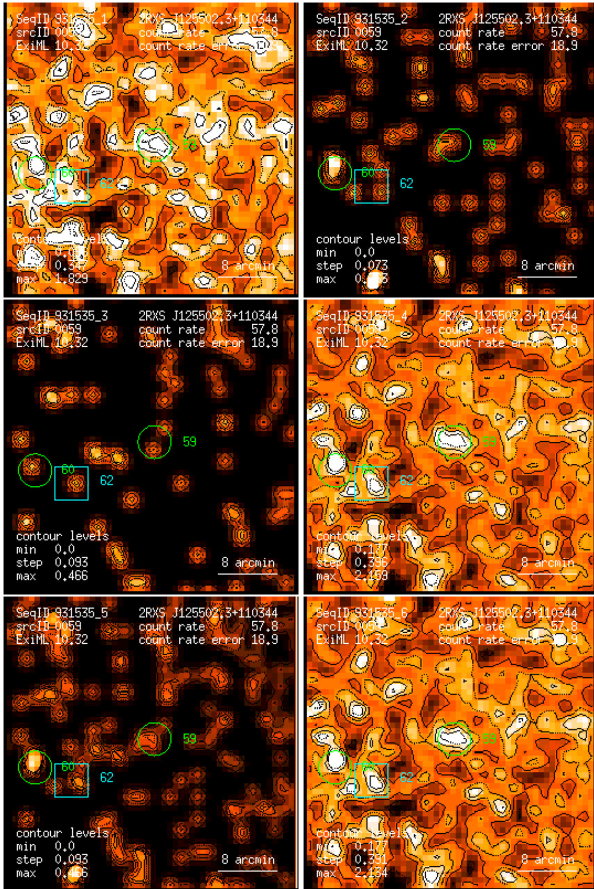
Figure 59: RASS 931535: detection 0059: band rate images, Gaussian filter: (1) PSPC channels 11 – 41, (2) 52 – 90, (3) 91 – 201, (4) 11 – 235, (5) 52 – 201, (6) 11 – 201. Broad band rates in counts/ks. Band rate contour levels in counts/ks/arcmin 2 .
