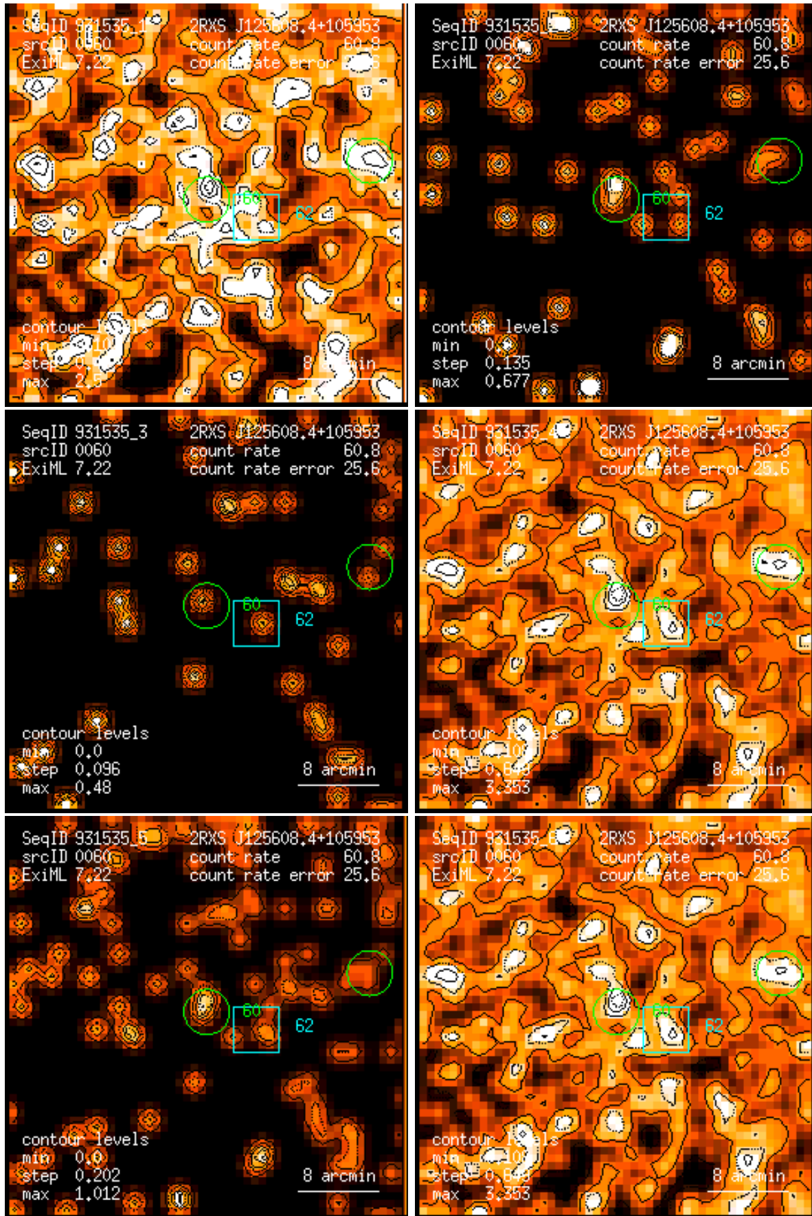
Figure 60: RASS 931535: detection 0060: band rate images, Gaussian filter: (1) PSPC channels 11 – 41, (2) 52 – 90, (3) 91 – 201, (4) 11 – 235, (5) 52 – 201, (6) 11 – 201. Broad band rates in counts/ks. Band rate contour levels in counts/ks/arcmin 2 .
