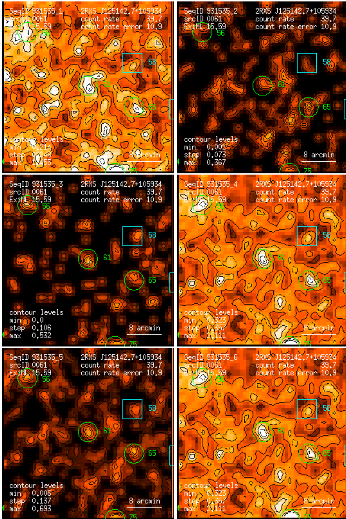
Figure 61: RASS 931535: detection 0061: band rate images, Gaussian filter: (1) PSPC channels 11 – 41, (2) 52 – 90, (3) 91 – 201, (4) 11 – 235, (5) 52 – 201, (6) 11 – 201. Broad band rates in counts/ks. Band rate contour levels in counts/ks/arcmin 2 .
