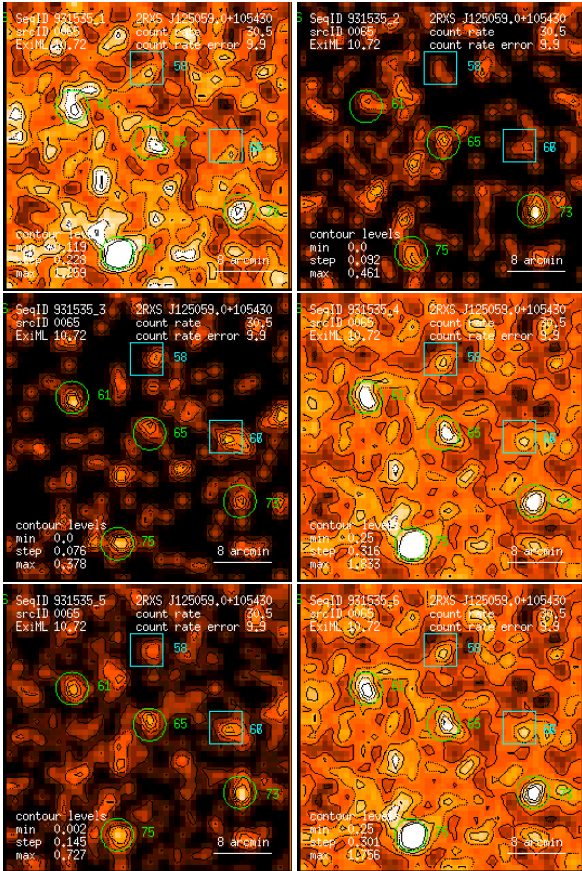
Figure 65: RASS 931535: detection 0065: band rate images, Gaussian filter: (1) PSPC channels 11 – 41, (2) 52 – 90, (3) 91 – 201, (4) 11 – 235, (5) 52 – 201, (6) 11 – 201. Broad band rates in counts/ks. Band rate contour levels in counts/ks/arcmin 2 .
