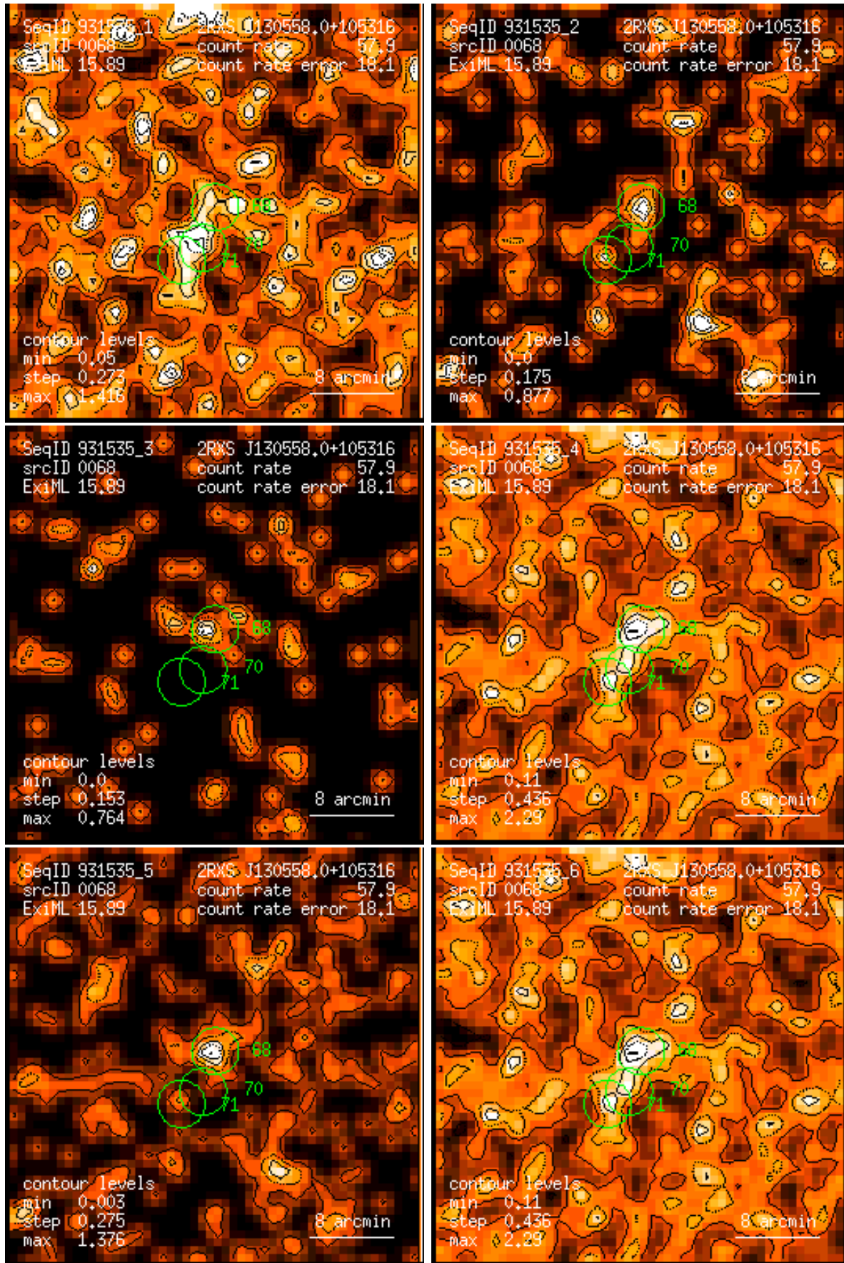
Figure 68: RASS 931535: detection 0068: band rate images, Gaussian filter: (1) PSPC channels 11 – 41, (2) 52 – 90, (3) 91 – 201, (4) 11 – 235, (5) 52 – 201, (6) 11 – 201. Broad band rates in counts/ks. Band rate contour levels in counts/ks/arcmin 2 .
