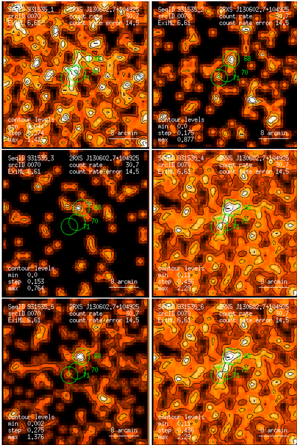
Figure 70: RASS 931535: detection 0070: band rate images, Gaussian filter: (1) PSPC channels 11 – 41, (2) 52 – 90, (3) 91 – 201, (4) 11 – 235, (5) 52 – 201, (6) 11 – 201. Broad band rates in counts/ks. Band rate contour levels in counts/ks/arcmin 2 .
