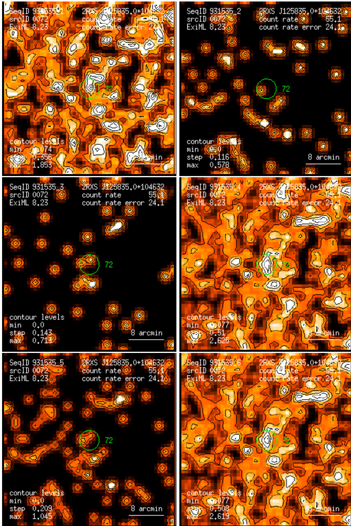
Figure 72: RASS 931535: detection 0072: band rate images, Gaussian filter: (1) PSPC channels 11 – 41, (2) 52 – 90, (3) 91 – 201, (4) 11 – 235, (5) 52 – 201, (6) 11 – 201. Broad band rates in counts/ks. Band rate contour levels in counts/ks/arcmin 2 .
