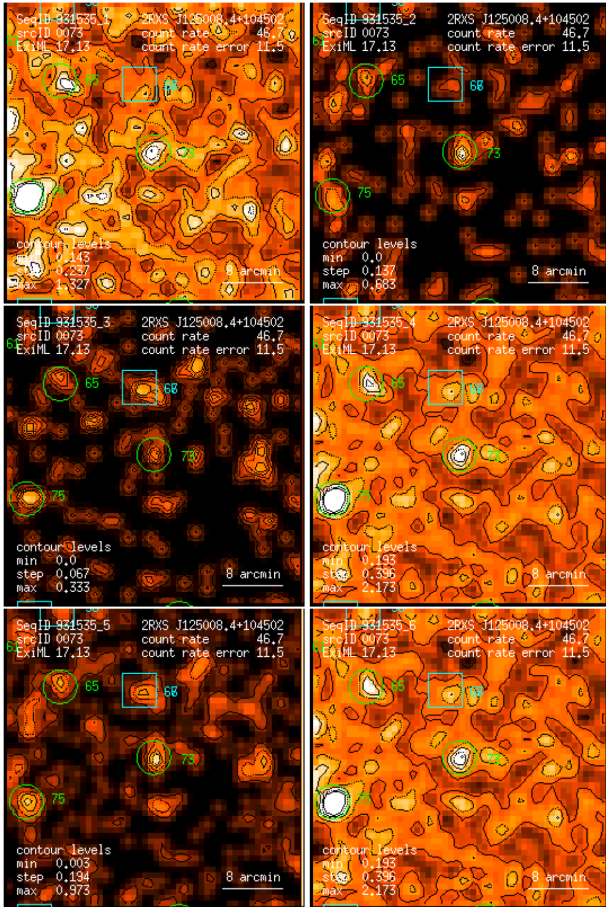
Figure 73: RASS 931535: detection 0073: band rate images, Gaussian filter: (1) PSPC channels 11 – 41, (2) 52 – 90, (3) 91 – 201, (4) 11 – 235, (5) 52 – 201, (6) 11 – 201. Broad band rates in counts/ks. Band rate contour levels in counts/ks/arcmin 2 .
