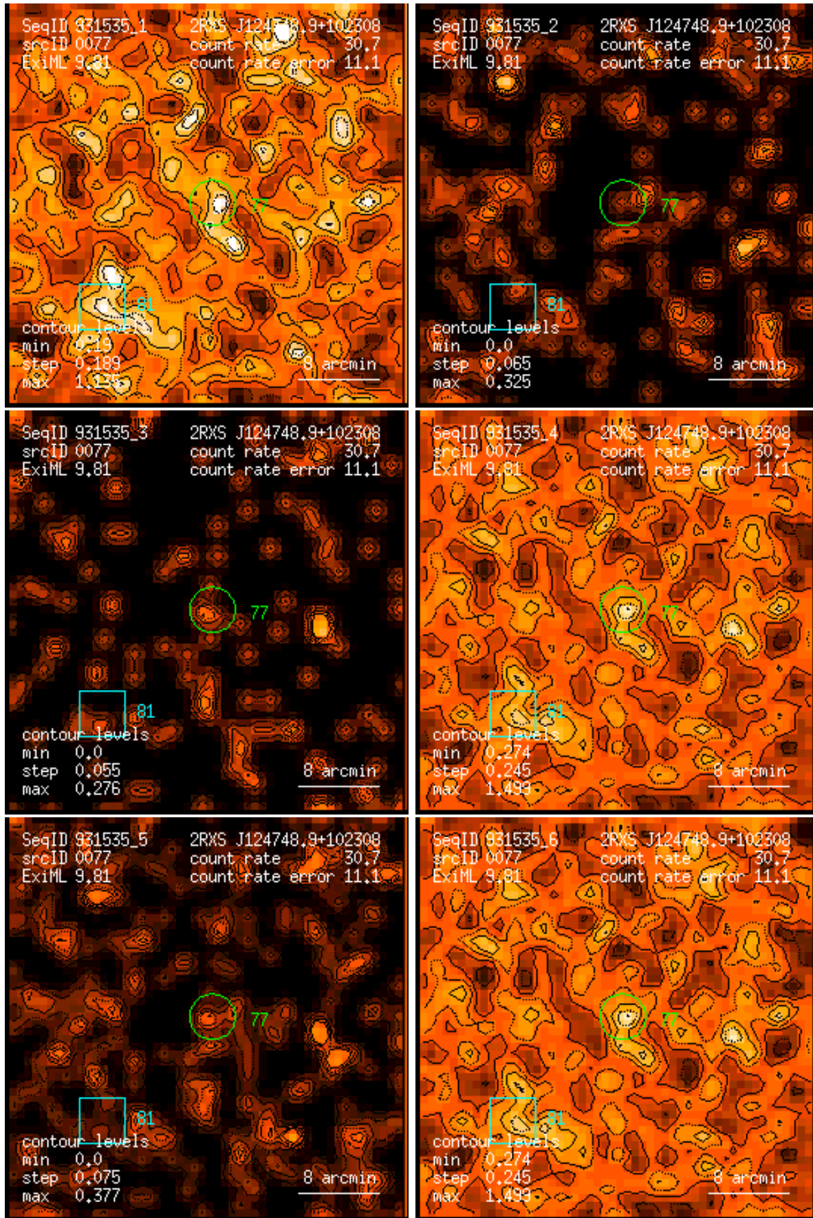
Figure 77: RASS 931535: detection 0077: band rate images, Gaussian filter: (1) PSPC channels 11 – 41, (2) 52 – 90, (3) 91 – 201, (4) 11 – 235, (5) 52 – 201, (6) 11 – 201. Broad band rates in counts/ks. Band rate contour levels in counts/ks/arcmin 2 .
