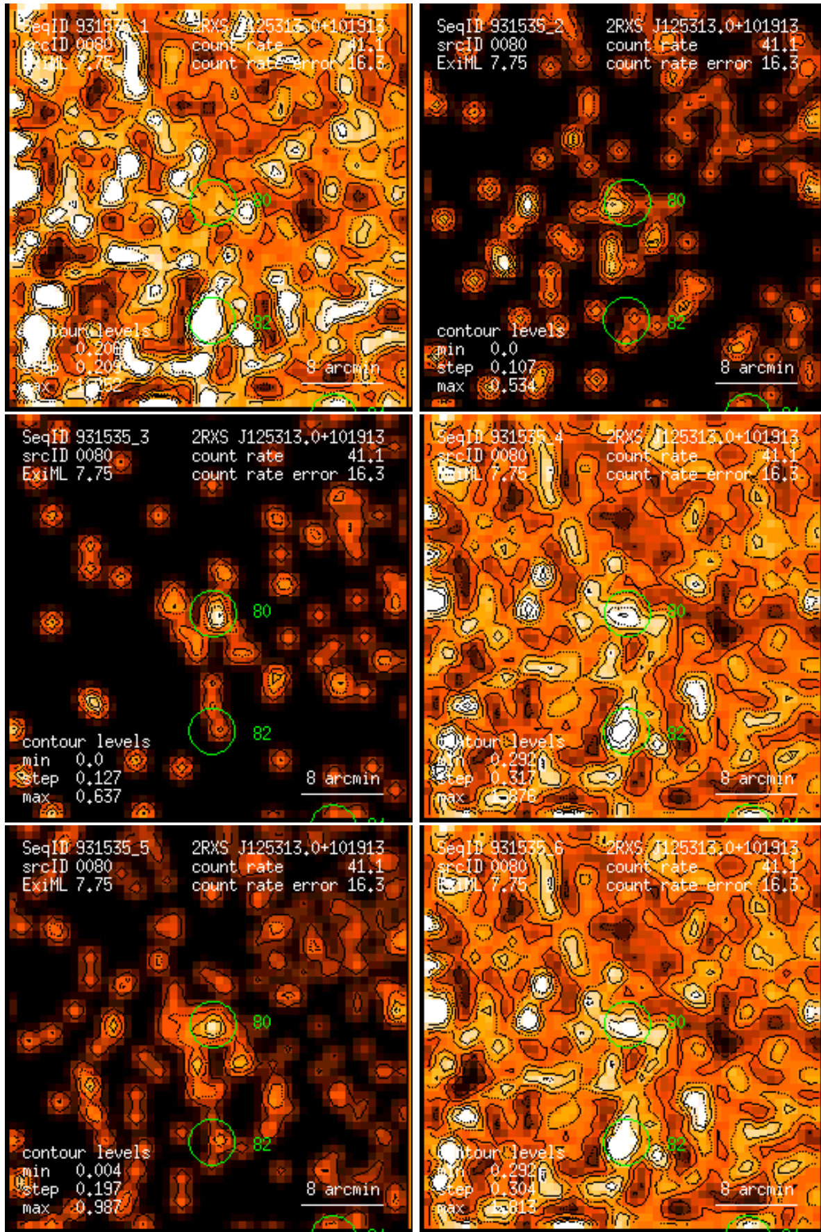
Figure 80: RASS 931535: detection 0080: band rate images, Gaussian filter: (1) PSPC channels 11 – 41, (2) 52 – 90, (3) 91 – 201, (4) 11 – 235, (5) 52 – 201, (6) 11 – 201. Broad band rates in counts/ks. Band rate contour levels in counts/ks/arcmin 2 .
